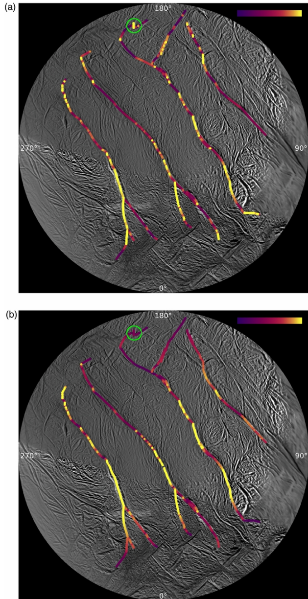
Figure 6. from How the Geysers, Tidal Stresses, and Thermal Emission across the South Polar Terrain of Enceladus are Related Porco, DiNino, & Nimmo 2014 AJ 148 45 doi:10.1088/0004-6256/148/3/45 https://dx.doi.org/10.1088/0004-6256/148/3/45 © 2014. The American Astronomical Society. All rights reserved.
