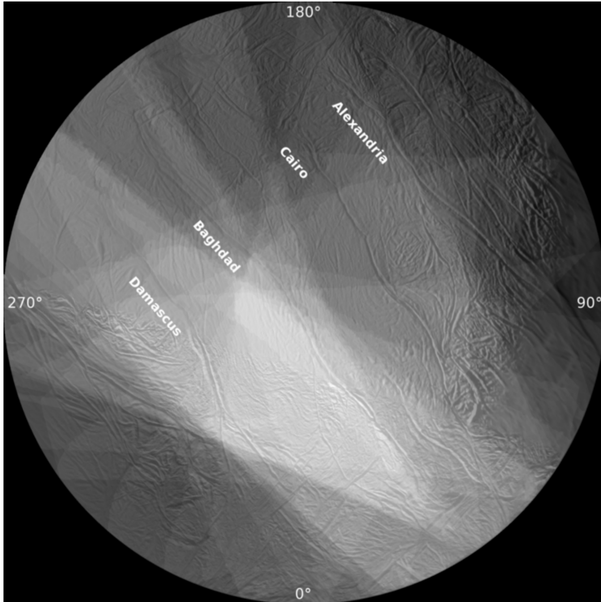
Figure 5. from How the Geysers, Tidal Stresses, and Thermal Emission across the South Polar Terrain of Enceladus are Related Porco, DiNino, & Nimmo 2014 AJ 148 45 doi:10.1088/0004-6256/148/3/45 https://dx.doi.org/10.1088/0004-6256/148/3/45 © 2014. The American Astronomical Society. All rights reserved.
