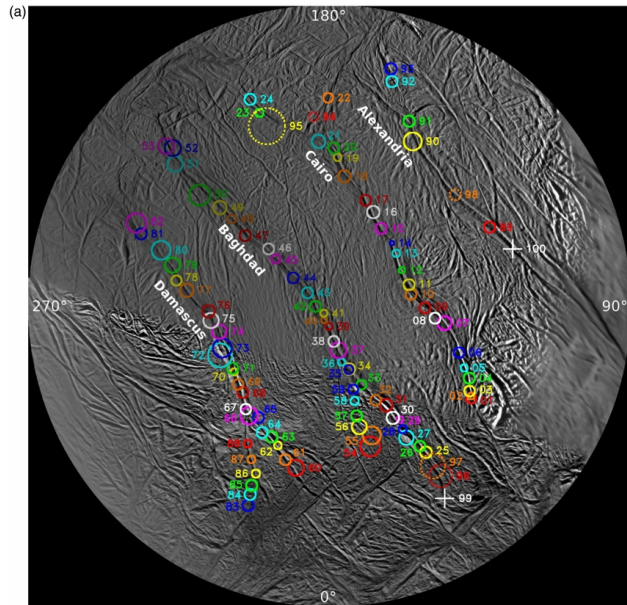
Figure 3. from How the Geysers, Tidal Stresses, and Thermal Emission across the South Polar Terrain of Enceladus are Related Porco, DiNino, & Nimmo 2014 AJ 148 45 doi:10.1088/0004-6256/148/3/45 https://dx.doi.org/10.1088/0004-6256/148/3/45 © 2014. The American Astronomical Society. All rights reserved.
