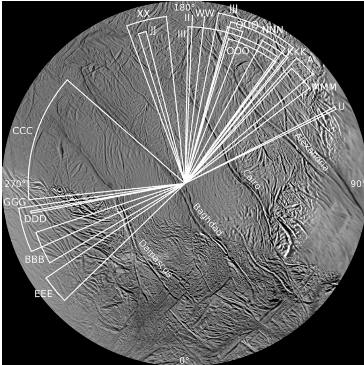
Figure 2. from How the Geysers, Tidal Stresses, and Thermal Emission across the South Polar Terrain of Enceladus are Related Porco, DiNino, & Nimmo 2014 AJ 148 45 doi:10.1088/0004-6256/148/3/45 https://dx.doi.org/10.1088/0004-6256/148/3/45 © 2014. The American Astronomical Society. All rights reserved.
