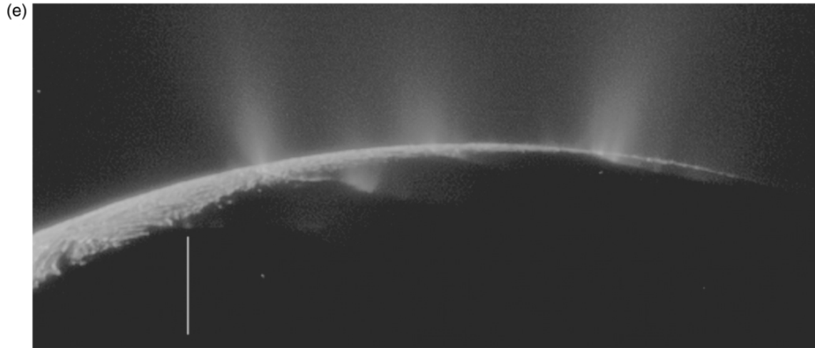
Figure 1. from How the Geysers, Tidal Stresses, and Thermal Emission across the South Polar Terrain of Enceladus are Related Porco, DiNino, & Nimmo 2014 AJ 148 45 doi:10.1088/0004-6256/148/3/45 https://dx.doi.org/10.1088/0004-6256/148/3/45 © 2014. The American Astronomical Society. All rights reserved.
