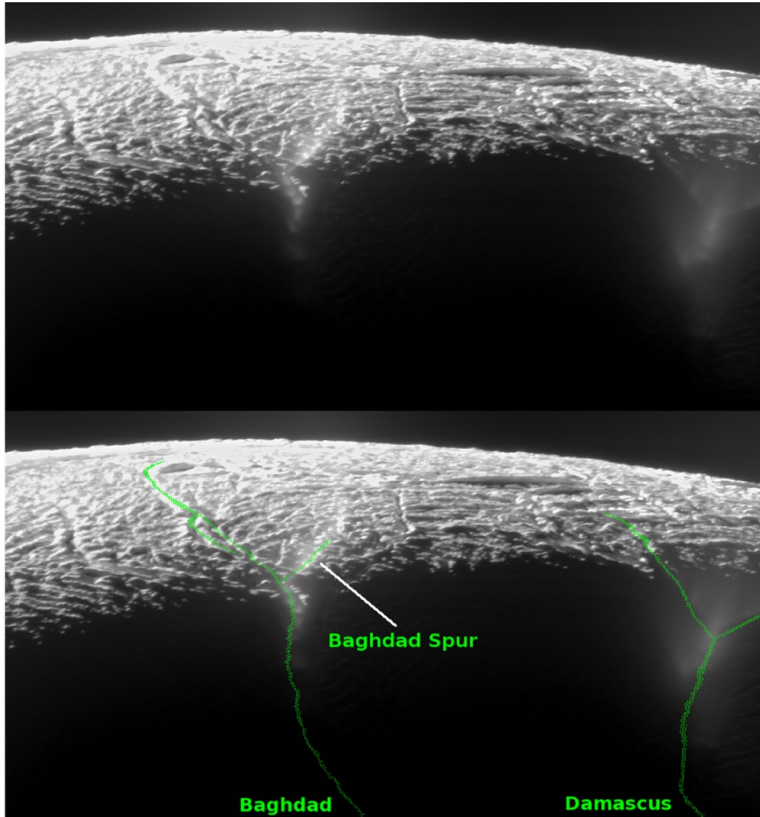
Figure 1. from How the Geysers, Tidal Stresses, and Thermal Emission across the South Polar Terrain of Enceladus are Related Porco, DiNino, & Nimmo 2014 AJ 148 45 doi:10.1088/0004-6256/148/3/45 https://dx.doi.org/10.1088/0004-6256/148/3/45 © 2014. The American Astronomical Society. All rights reserved.
