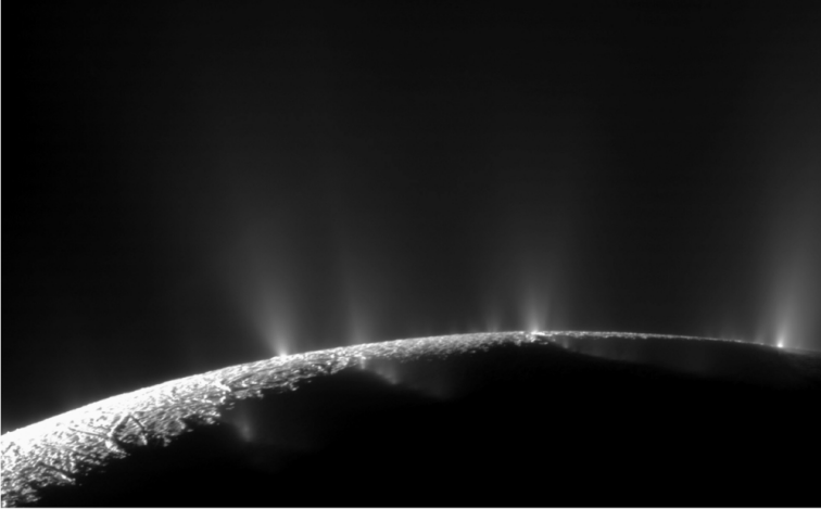
Figure 1. from How the Geysers, Tidal Stresses, and Thermal Emission across the South Polar Terrain of Enceladus are Related Porco, DiNino, & Nimmo 2014 AJ 148 45 doi:10.1088/0004-6256/148/3/45 https://dx.doi.org/10.1088/0004-6256/148/3/45 © 2014. The American Astronomical Society. All rights reserved.
