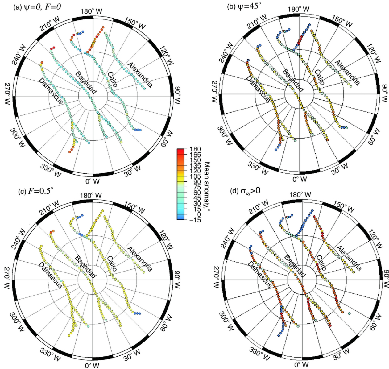
Figure 8. from Tidally Modulated Eruptions on Enceladus: Cassini ISS Observations and Models Nimmo, Porco, & Mitchell 2014 AJ 148 46 doi:10.1088/0004-6256/148/3/46 https://dx.doi.org/10.1088/0004-6256/148/3/46 © 2014. The American Astronomical Society. All rights reserved.
