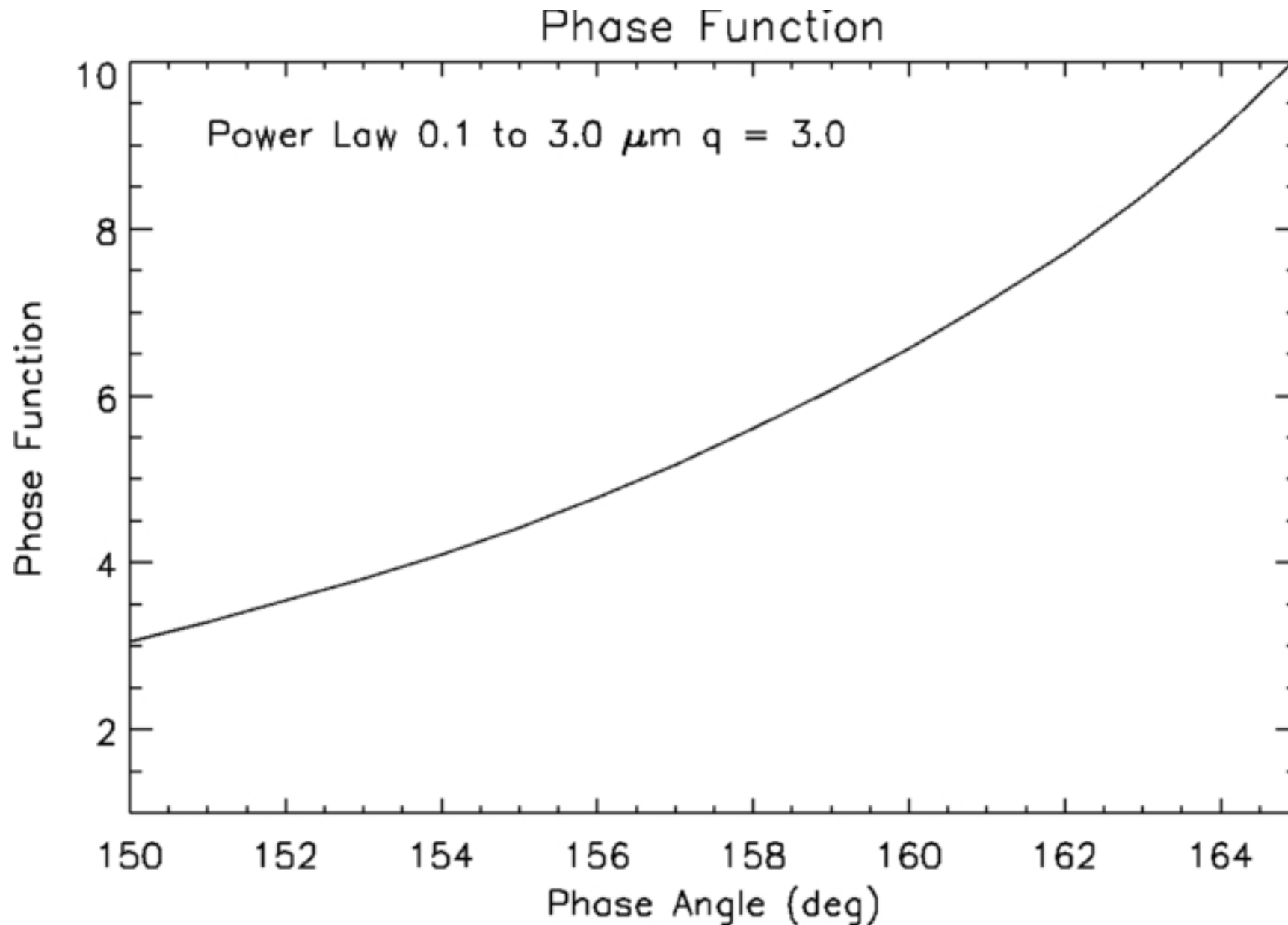
Figure 4. from Tidally Modulated Eruptions on Enceladus: Cassini ISS Observations and Models Nimmo, Porco, & Mitchell 2014 AJ 148 46 doi:10.1088/0004-6256/148/3/46 https://dx.doi.org/10.1088/0004-6256/148/3/46 © 2014. The American Astronomical Society. All rights reserved.
