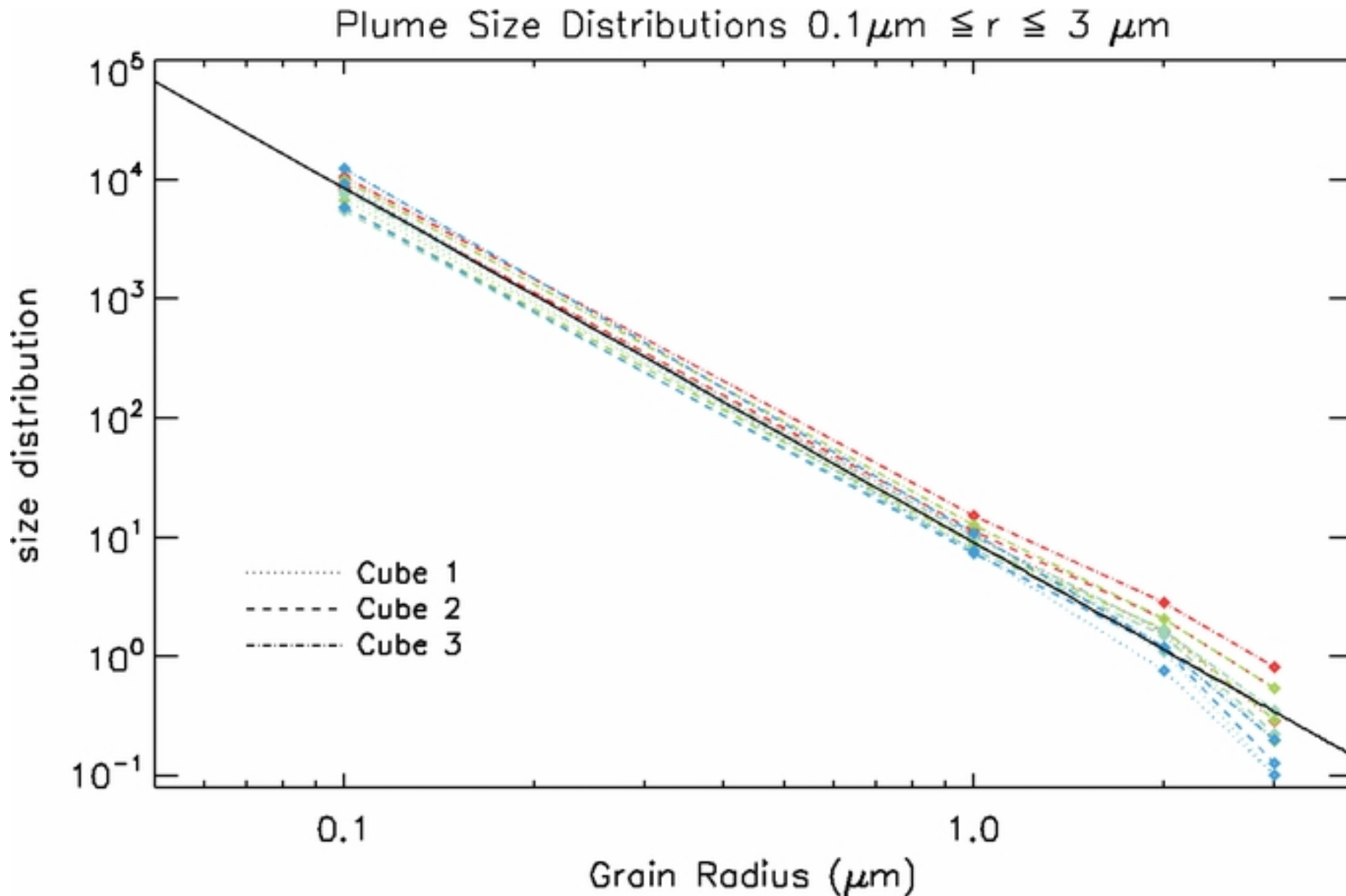
Figure 3. from Tidally Modulated Eruptions on Enceladus: Cassini ISS Observations and Models Nimmo, Porco, & Mitchell 2014 AJ 148 46 doi:10.1088/0004-6256/148/3/46 https://dx.doi.org/10.1088/0004-6256/148/3/46 © 2014. The American Astronomical Society. All rights reserved.
