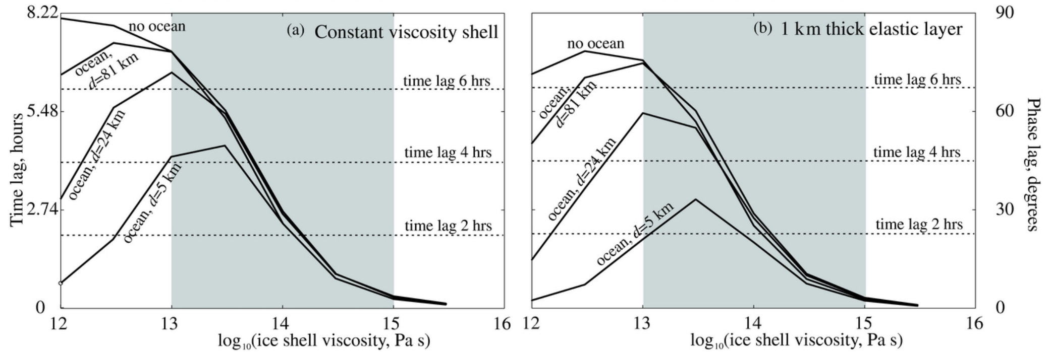
Figure 11. from Tidally Modulated Eruptions on Enceladus: Cassini ISS Observations and Models Nimmo, Porco, & Mitchell 2014 AJ 148 46 doi:10.1088/0004-6256/148/3/46 https://dx.doi.org/10.1088/0004-6256/148/3/46 © 2014. The American Astronomical Society. All rights reserved.
