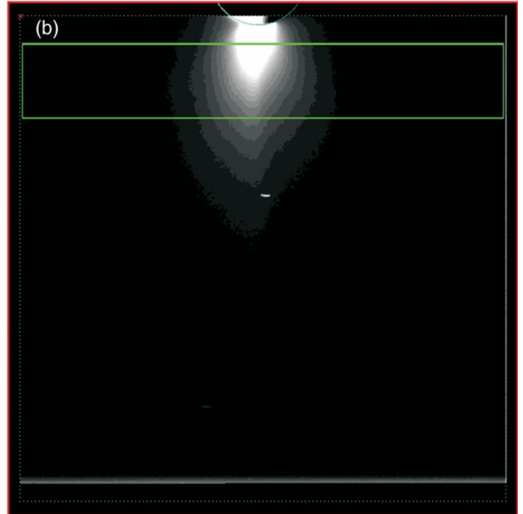
Figure 1. from Tidally Modulated Eruptions on Enceladus: Cassini ISS Observations and Models Nimmo, Porco, & Mitchell 2014 AJ 148 46 doi:10.1088/0004-6256/148/3/46 https://dx.doi.org/10.1088/0004-6256/148/3/46 © 2014. The American Astronomical Society. All rights reserved.
