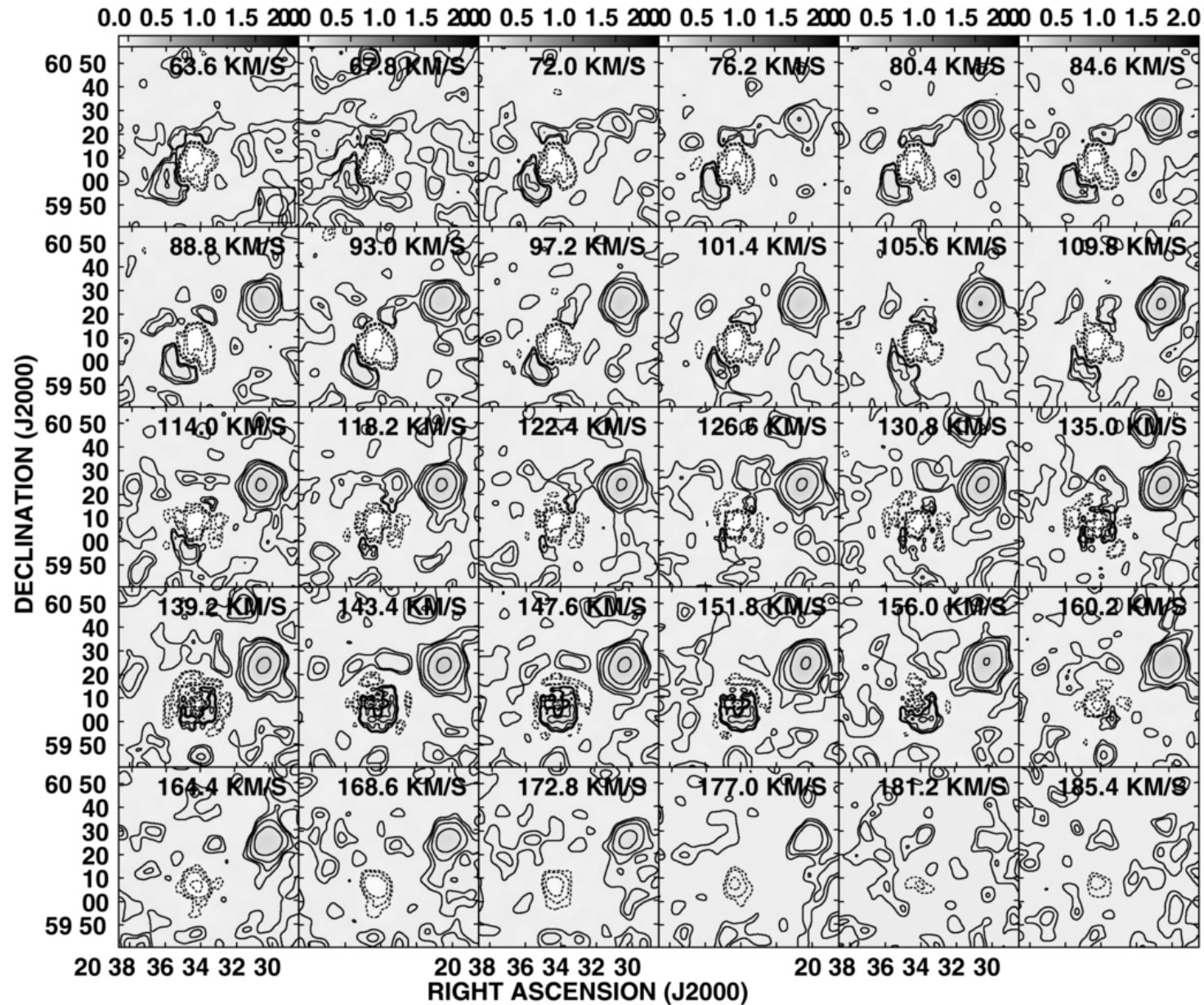
Figure 7. from Green Bank Telescope Observations of Low Column Density H I around NGC 2997 and NGC 6946 Pisano 2014 AJ 147 48 doi:10.1088/0004-6256/147/3/48 https://dx.doi.org/10.1088/0004-6256/147/3/48 © 2014. The American Astronomical Society. All rights reserved.
