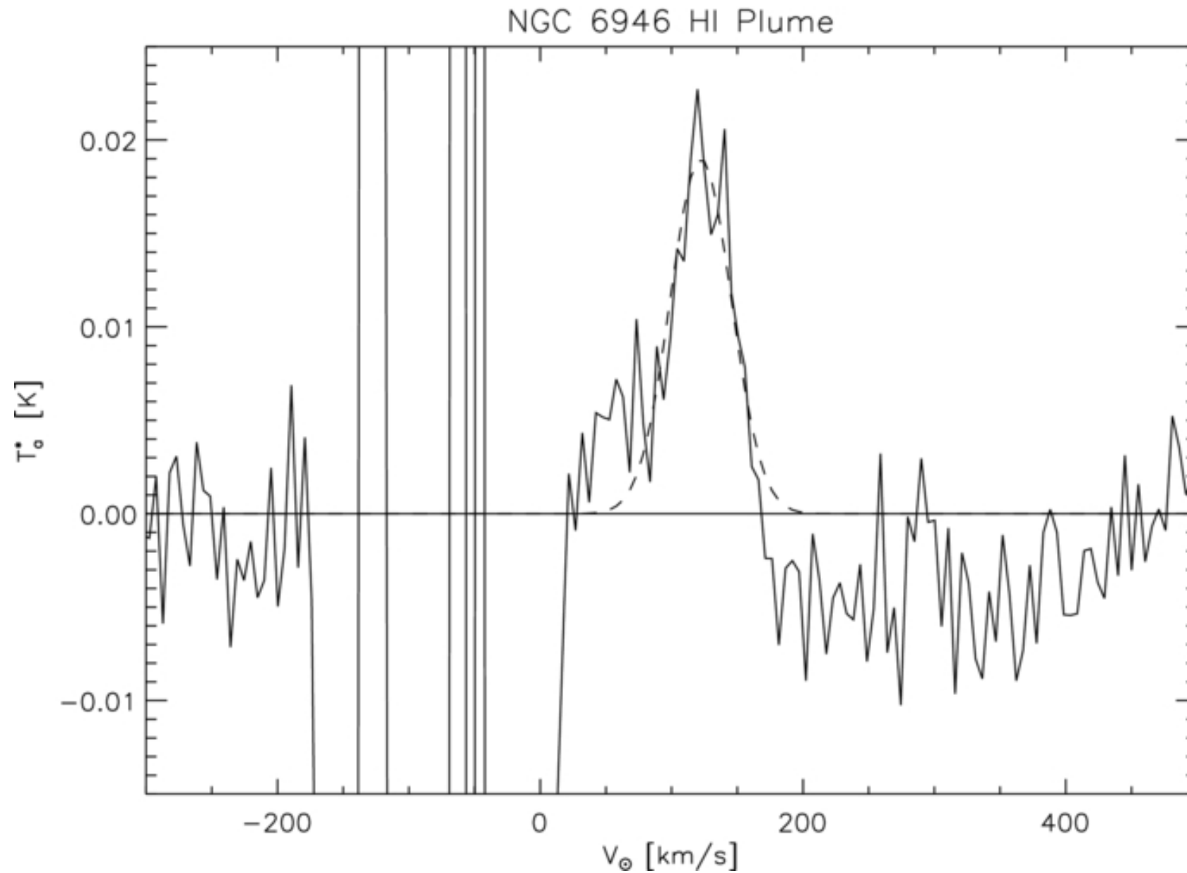
Figure 5. from Green Bank Telescope Observations of Low Column Density H I around NGC 2997 and NGC 6946 Pisano 2014 AJ 147 48 doi:10.1088/0004-6256/147/3/48 https://dx.doi.org/10.1088/0004-6256/147/3/48 © 2014. The American Astronomical Society. All rights reserved.
