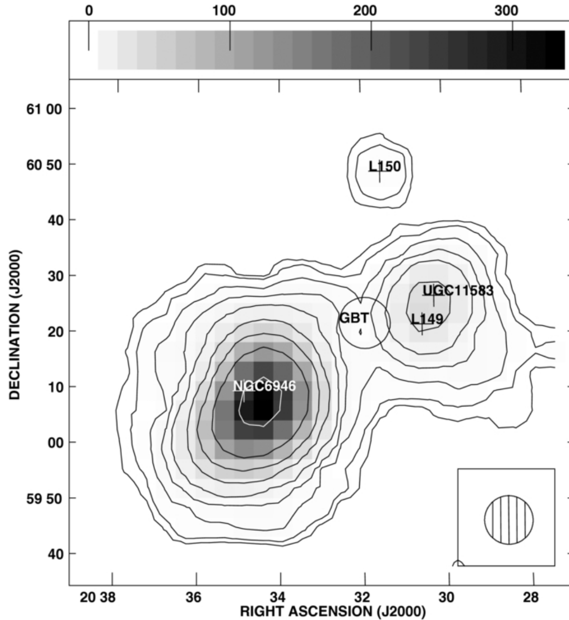
Figure 4. from Green Bank Telescope Observations of Low Column Density H I around NGC 2997 and NGC 6946 Pisano 2014 AJ 147 48 doi:10.1088/0004-6256/147/3/48 https://dx.doi.org/10.1088/0004-6256/147/3/48 © 2014. The American Astronomical Society. All rights reserved.
