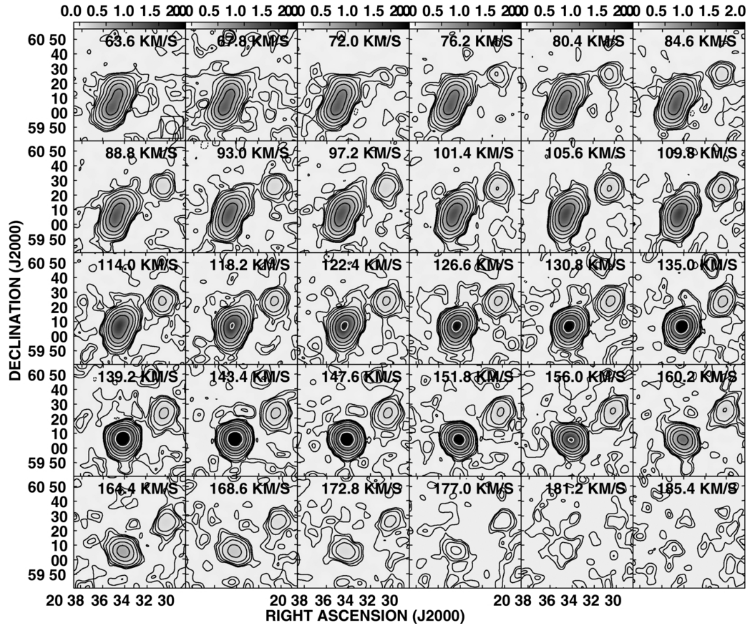
Figure 3. from Green Bank Telescope Observations of Low Column Density H I around NGC 2997 and NGC 6946 Pisano 2014 AJ 147 48 doi:10.1088/0004-6256/147/3/48 https://dx.doi.org/10.1088/0004-6256/147/3/48 © 2014. The American Astronomical Society. All rights reserved.
