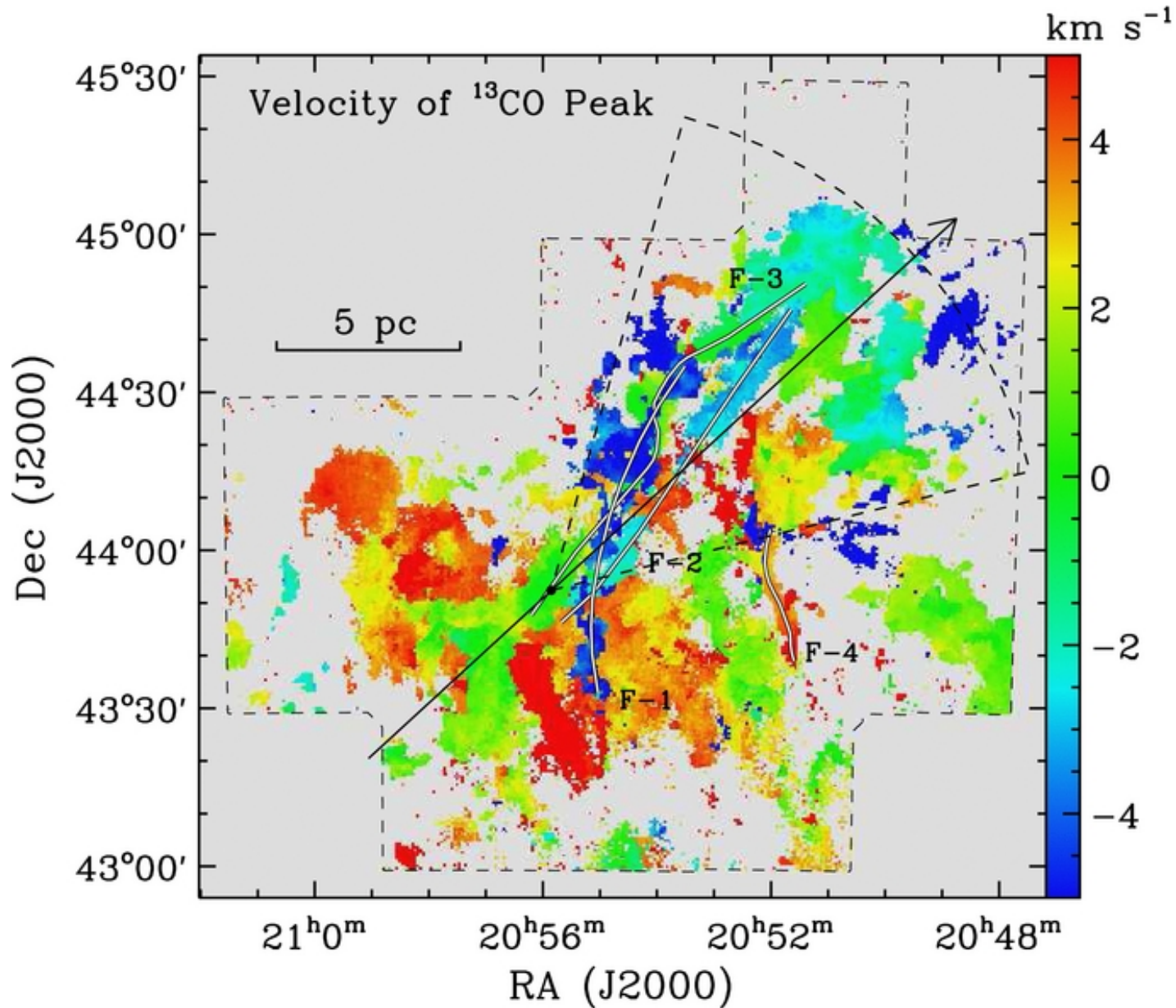
Figure 7. from Molecular Clouds in the North American and Pelican Nebulae: Structures Zhang, Xu, & Yang 2014 AJ 147 46 doi:10.1088/0004-6256/147/3/46 https://dx.doi.org/10.1088/0004-6256/147/3/46 © 2014. The American Astronomical Society. All rights reserved.
