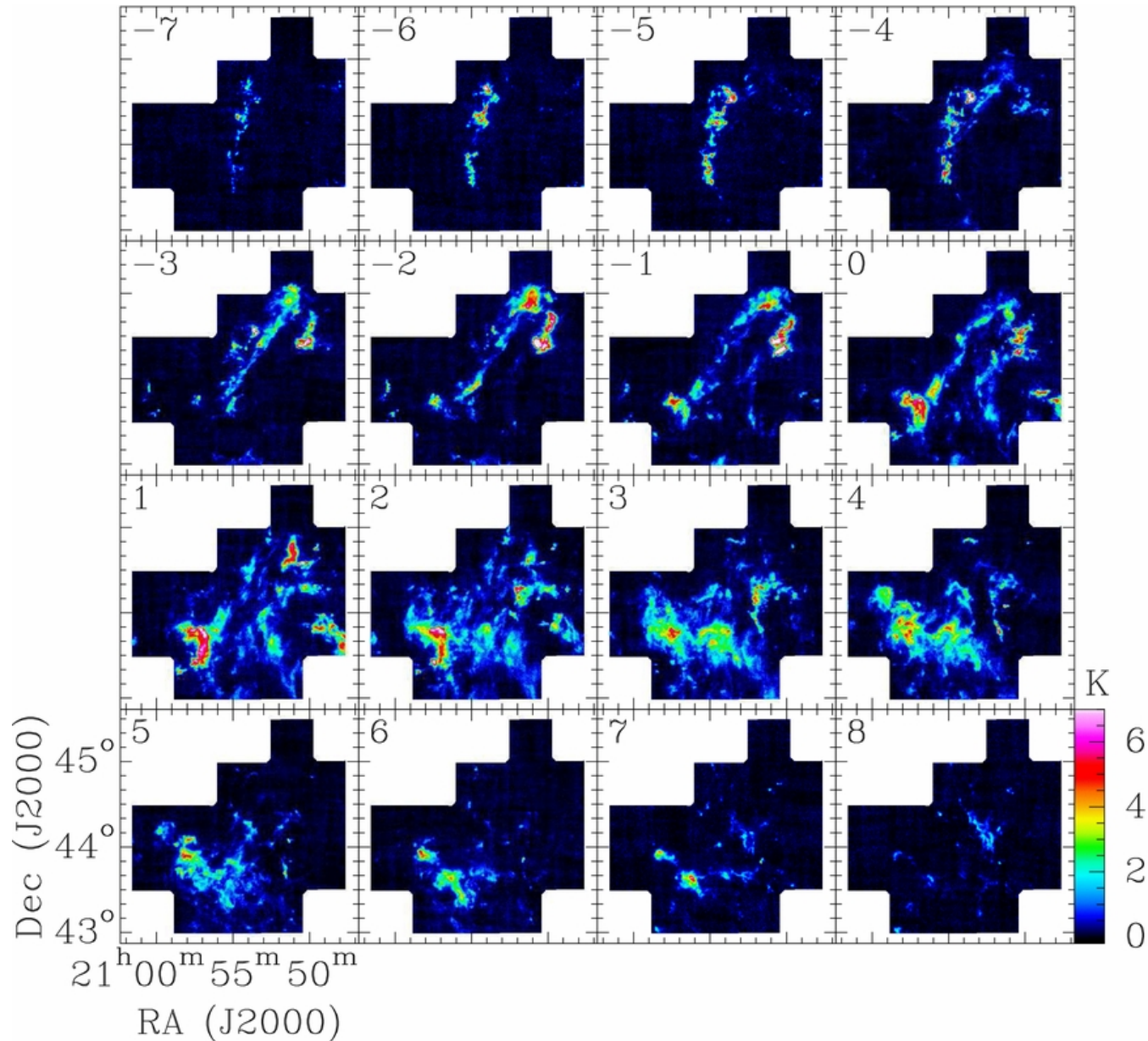
Figure 6. from Molecular Clouds in the North American and Pelican Nebulae: Structures Zhang, Xu, & Yang 2014 AJ 147 46 doi:10.1088/0004-6256/147/3/46 https://dx.doi.org/10.1088/0004-6256/147/3/46 © 2014. The American Astronomical Society. All rights reserved.
