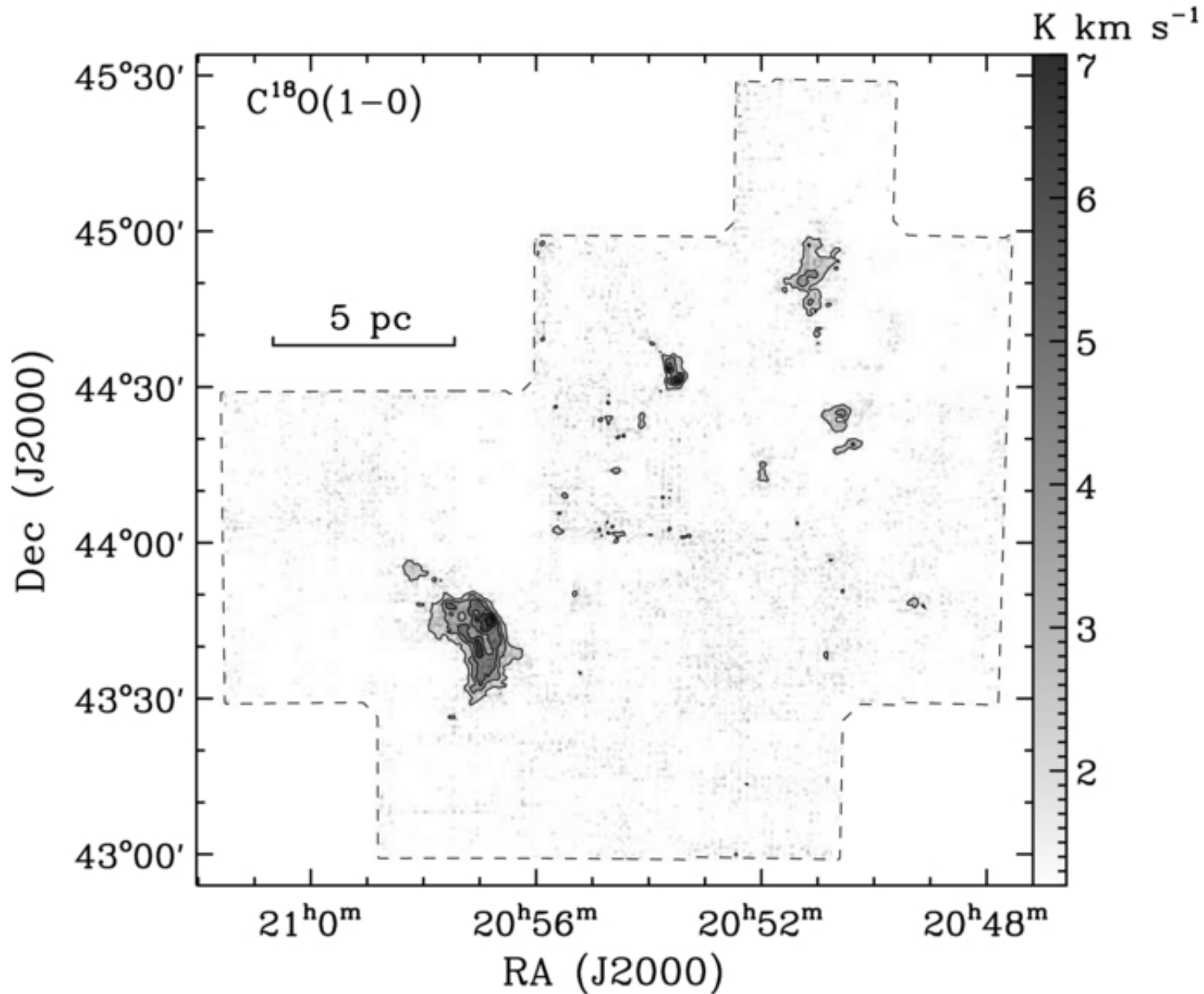
Figure 5. from Molecular Clouds in the North American and Pelican Nebulae: Structures Zhang, Xu, & Yang 2014 AJ 147 46 doi:10.1088/0004-6256/147/3/46 https://dx.doi.org/10.1088/0004-6256/147/3/46 © 2014. The American Astronomical Society. All rights reserved.
