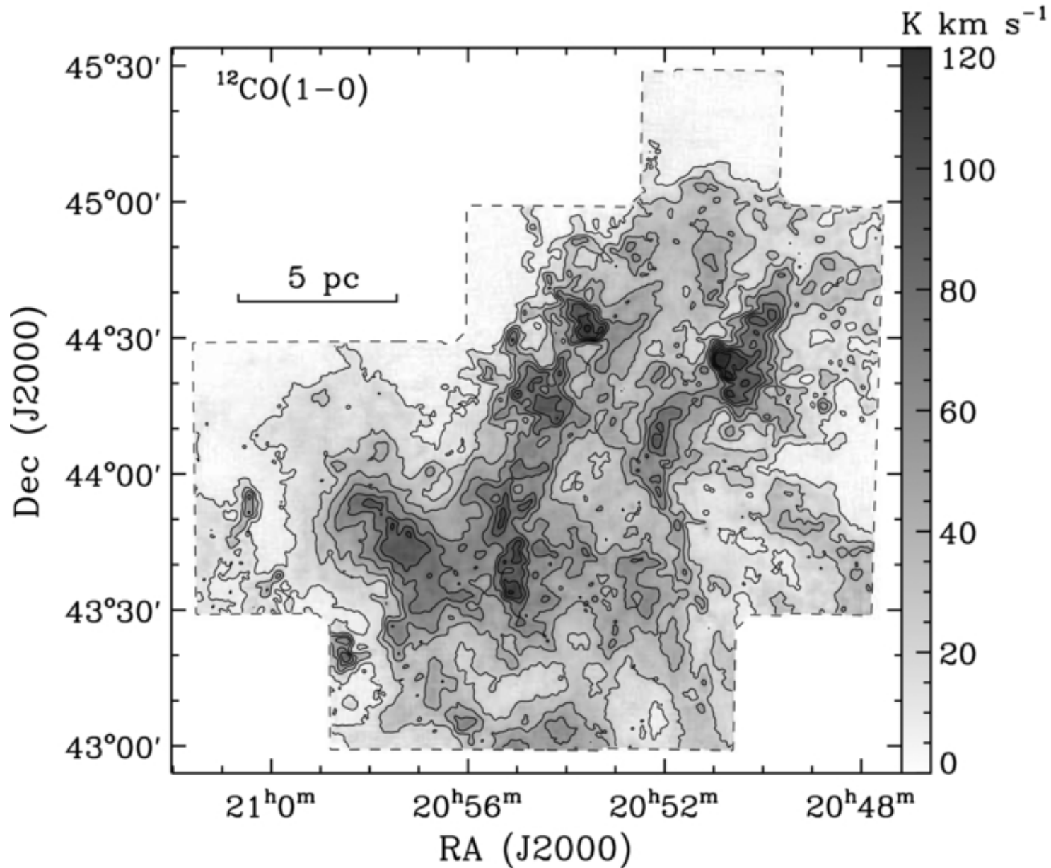
Figure 3. from Molecular Clouds in the North American and Pelican Nebulae: Structures Zhang, Xu, & Yang 2014 AJ 147 46 doi:10.1088/0004-6256/147/3/46 https://dx.doi.org/10.1088/0004-6256/147/3/46 © 2014. The American Astronomical Society. All rights reserved.
