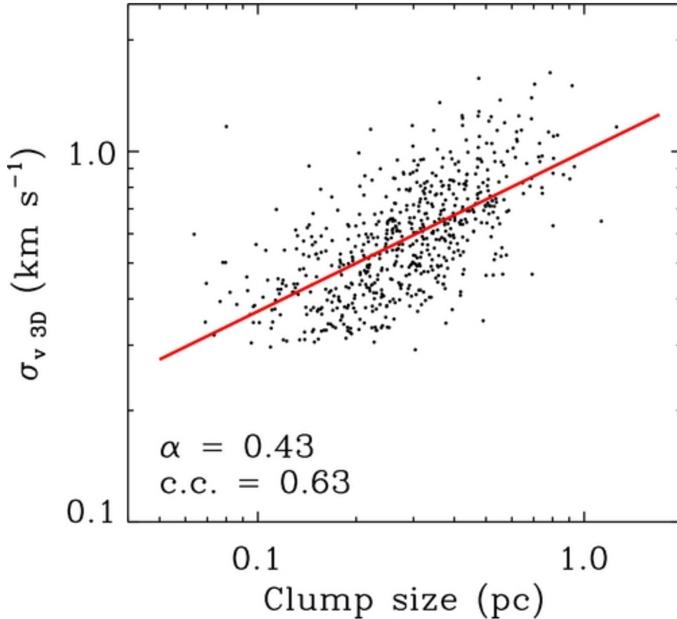
Figure 24. from Molecular Clouds in the North American and Pelican Nebulae: Structures Zhang, Xu, & Yang 2014 AJ 147 46 doi:10.1088/0004-6256/147/3/46 https://dx.doi.org/10.1088/0004-6256/147/3/46 © 2014. The American Astronomical Society. All rights reserved.
