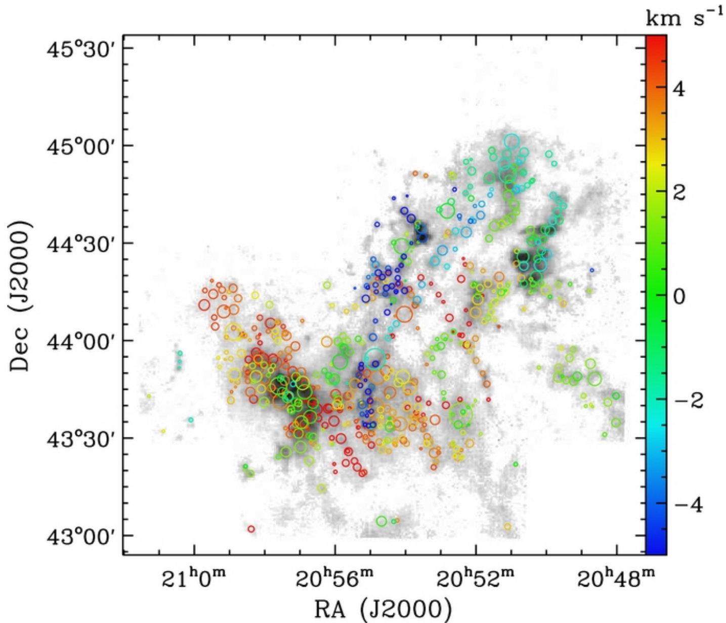
Figure 19. from Molecular Clouds in the North American and Pelican Nebulae: Structures Zhang, Xu, & Yang 2014 AJ 147 46 doi:10.1088/0004-6256/147/3/46 https://dx.doi.org/10.1088/0004-6256/147/3/46 © 2014. The American Astronomical Society. All rights reserved.
