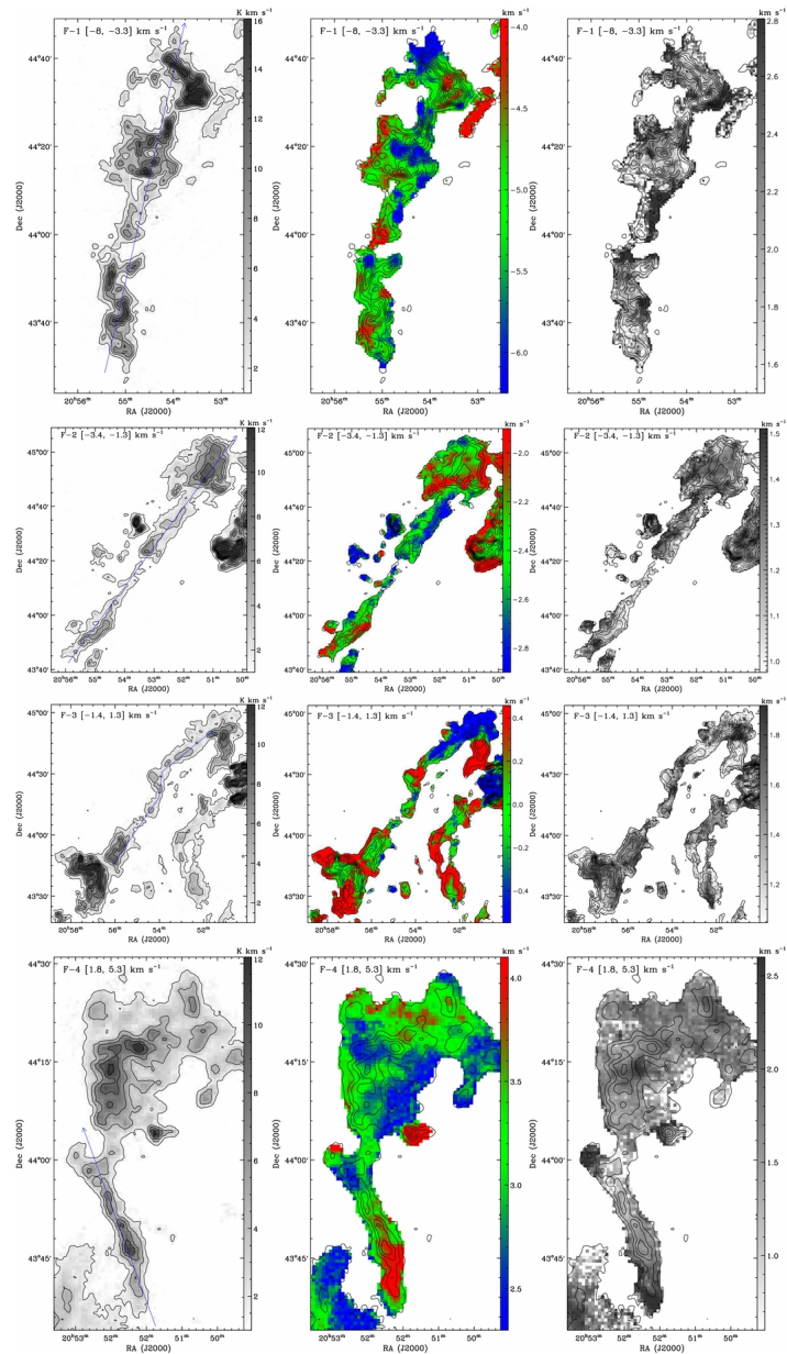
Figure 16. from Molecular Clouds in the North American and Pelican Nebulae: Structures Zhang, Xu, & Yang 2014 AJ 147 46 doi:10.1088/0004-6256/147/3/46 https://dx.doi.org/10.1088/0004-6256/147/3/46 © 2014. The American Astronomical Society. All rights reserved.
