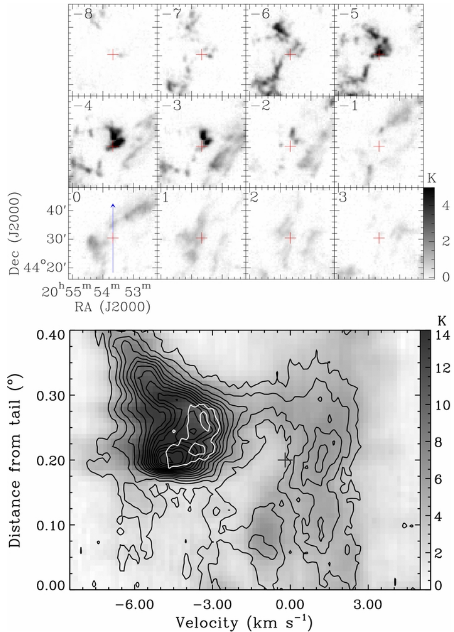
Figure 15. from Molecular Clouds in the North American and Pelican Nebulae: Structures Zhang, Xu, & Yang 2014 AJ 147 46 doi:10.1088/0004-6256/147/3/46 https://dx.doi.org/10.1088/0004-6256/147/3/46 © 2014. The American Astronomical Society. All rights reserved.
