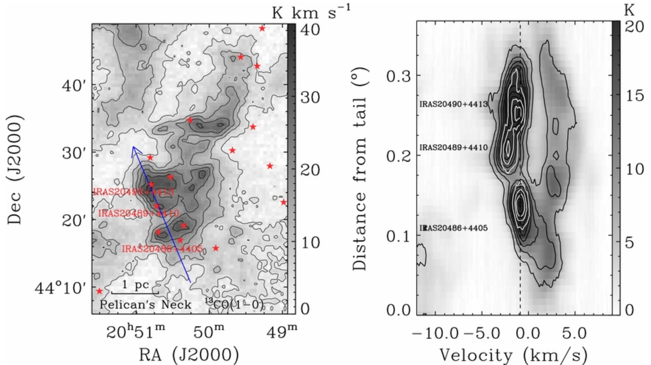
Figure 14. from Molecular Clouds in the North American and Pelican Nebulae: Structures Zhang, Xu, & Yang 2014 AJ 147 46 doi:10.1088/0004-6256/147/3/46 https://dx.doi.org/10.1088/0004-6256/147/3/46 © 2014. The American Astronomical Society. All rights reserved.
