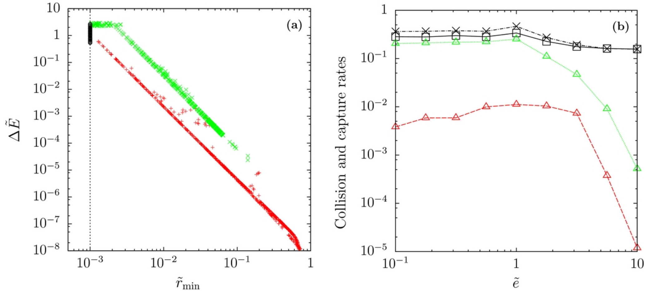
Figure 10. from Capture of Planetesimals by Gas Drag from Circumplanetary Disks Fujita et al. 2013 AJ 146 140 doi:10.1088/0004-6256/146/6/140 https://dx.doi.org/10.1088/0004-6256/146/6/140 © 2013. The American Astronomical Society. All rights reserved.
