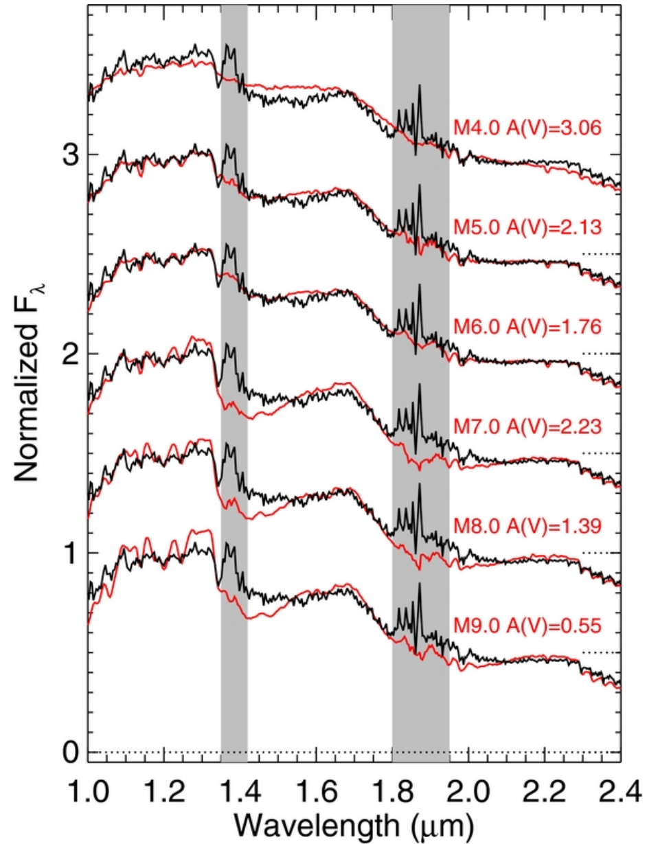
Figure 9. from HH 222: A Giant Herbig-Haro Flow from the Quadruple System V380 Ori Reipurth et al. 2013 AJ 146 118 doi:10.1088/0004-6256/146/5/118 https://dx.doi.org/10.1088/0004-6256/146/5/118 © 2013. The American Astronomical Society. All rights reserved.
