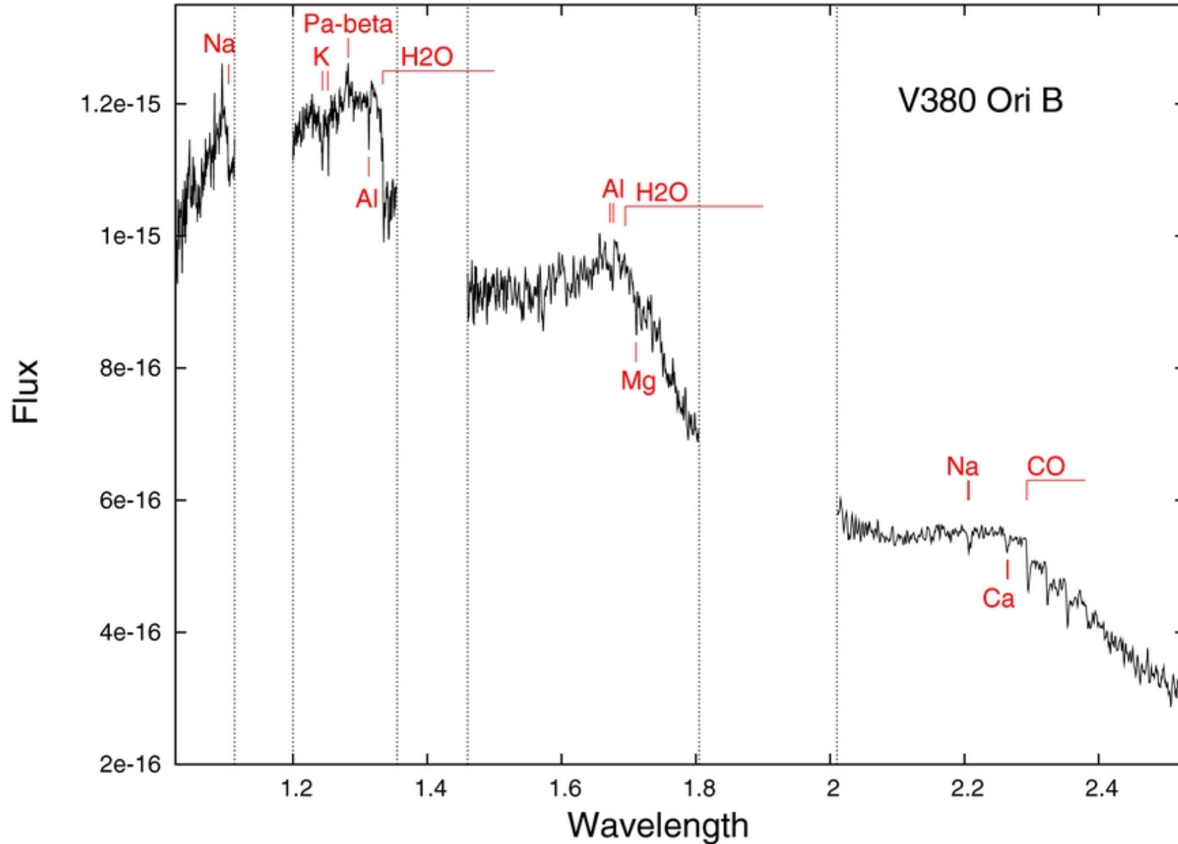
Figure 8. from HH 222: A Giant Herbig-Haro Flow from the Quadruple System V380 Ori Reipurth et al. 2013 AJ 146 118 doi:10.1088/0004-6256/146/5/118 https://dx.doi.org/10.1088/0004-6256/146/5/118 © 2013. The American Astronomical Society. All rights reserved.
