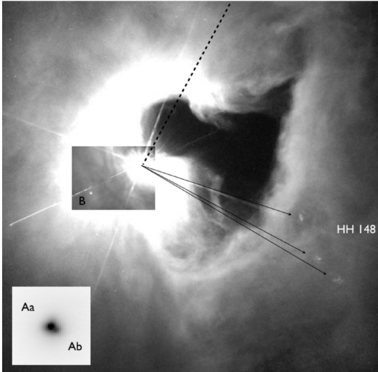
Figure 6. from HH 222: A Giant Herbig-Haro Flow from the Quadruple System V380 Ori Reipurth et al. 2013 AJ 146 118 doi:10.1088/0004-6256/146/5/118 https://dx.doi.org/10.1088/0004-6256/146/5/118 © 2013. The American Astronomical Society. All rights reserved.
