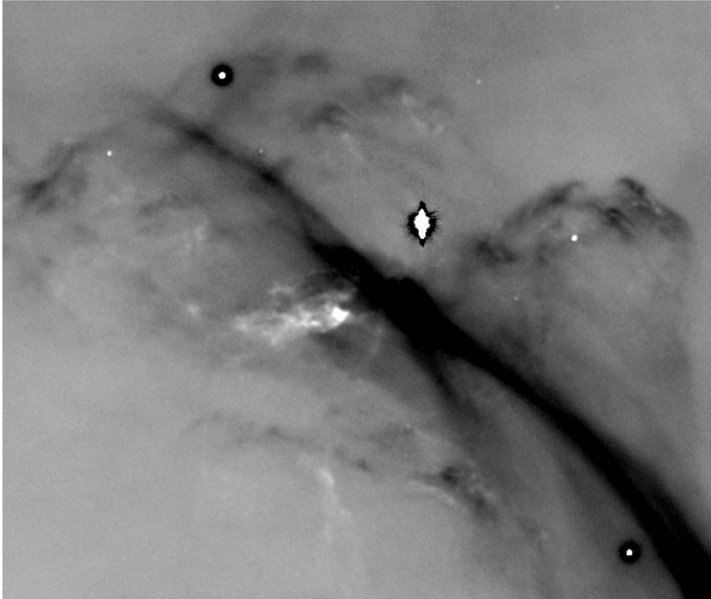
Figure 2. from HH 222: A Giant Herbig-Haro Flow from the Quadruple System V380 Ori Reipurth et al. 2013 AJ 146 118 doi:10.1088/0004-6256/146/5/118 https://dx.doi.org/10.1088/0004-6256/146/5/118 © 2013. The American Astronomical Society. All rights reserved.
