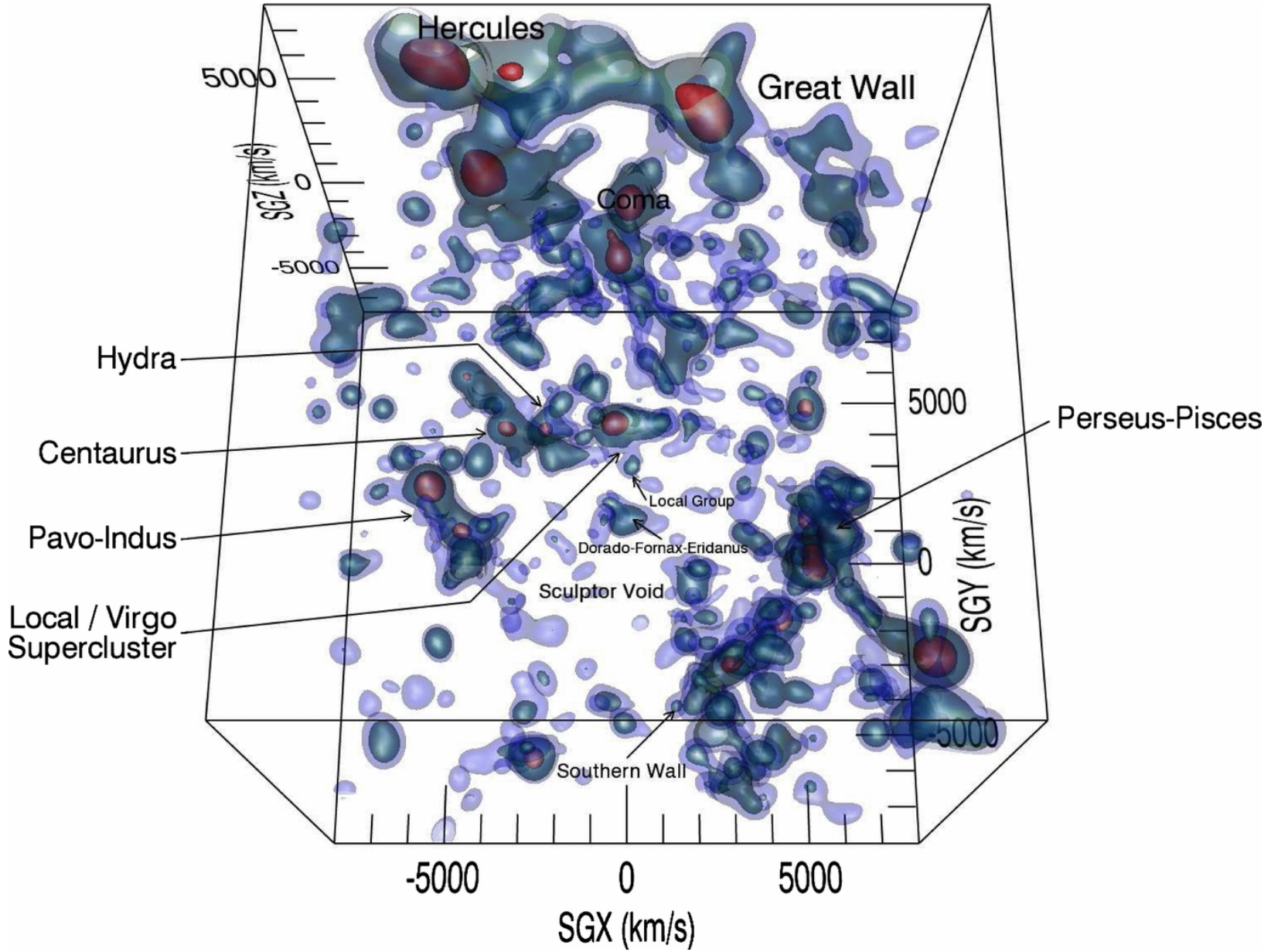
Figure 9. from Cosmography of the Local Universe Courtois et al. 2013 AJ 146 69 doi:10.1088/0004-6256/146/3/69 https://dx.doi.org/10.1088/0004-6256/146/3/69 © 2013. The American Astronomical Society. All rights reserved.
