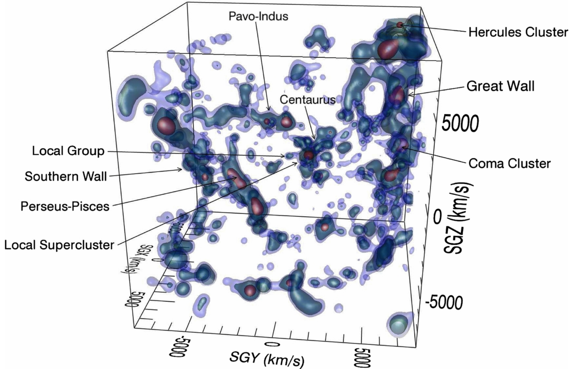
Figure 8. from Cosmography of the Local Universe Courtois et al. 2013 AJ 146 69 doi:10.1088/0004-6256/146/3/69 https://dx.doi.org/10.1088/0004-6256/146/3/69 © 2013. The American Astronomical Society. All rights reserved.
