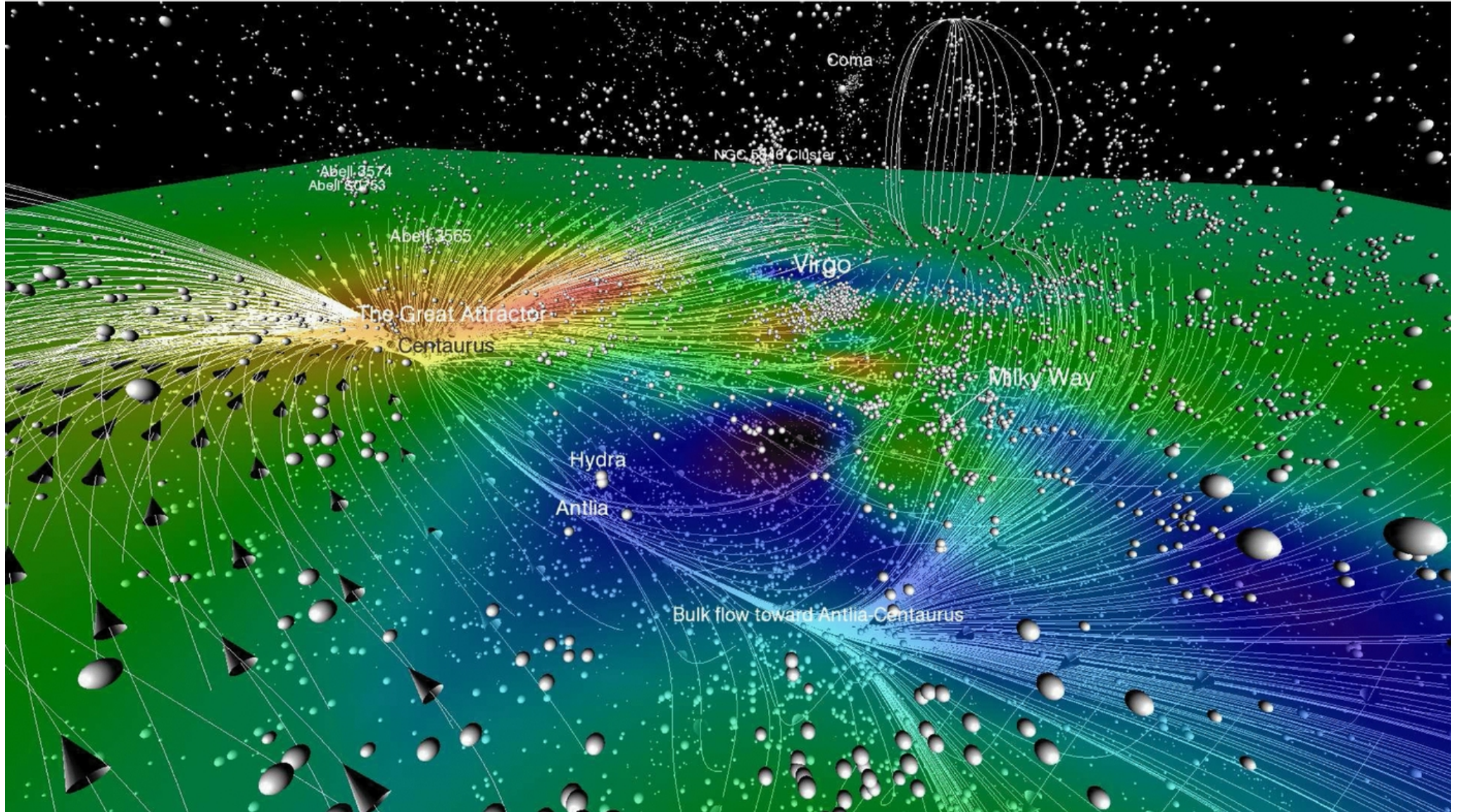
Figure 22. from Cosmography of the Local Universe Courtois et al. 2013 AJ 146 69 doi:10.1088/0004-6256/146/3/69 https://dx.doi.org/10.1088/0004-6256/146/3/69 © 2013. The American Astronomical Society. All rights reserved.
