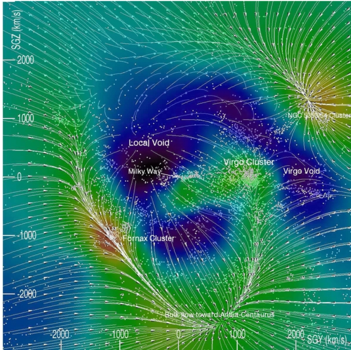
Figure 21. from Cosmography of the Local Universe Courtois et al. 2013 AJ 146 69 doi:10.1088/0004-6256/146/3/69 https://dx.doi.org/10.1088/0004-6256/146/3/69 © 2013. The American Astronomical Society. All rights reserved.
