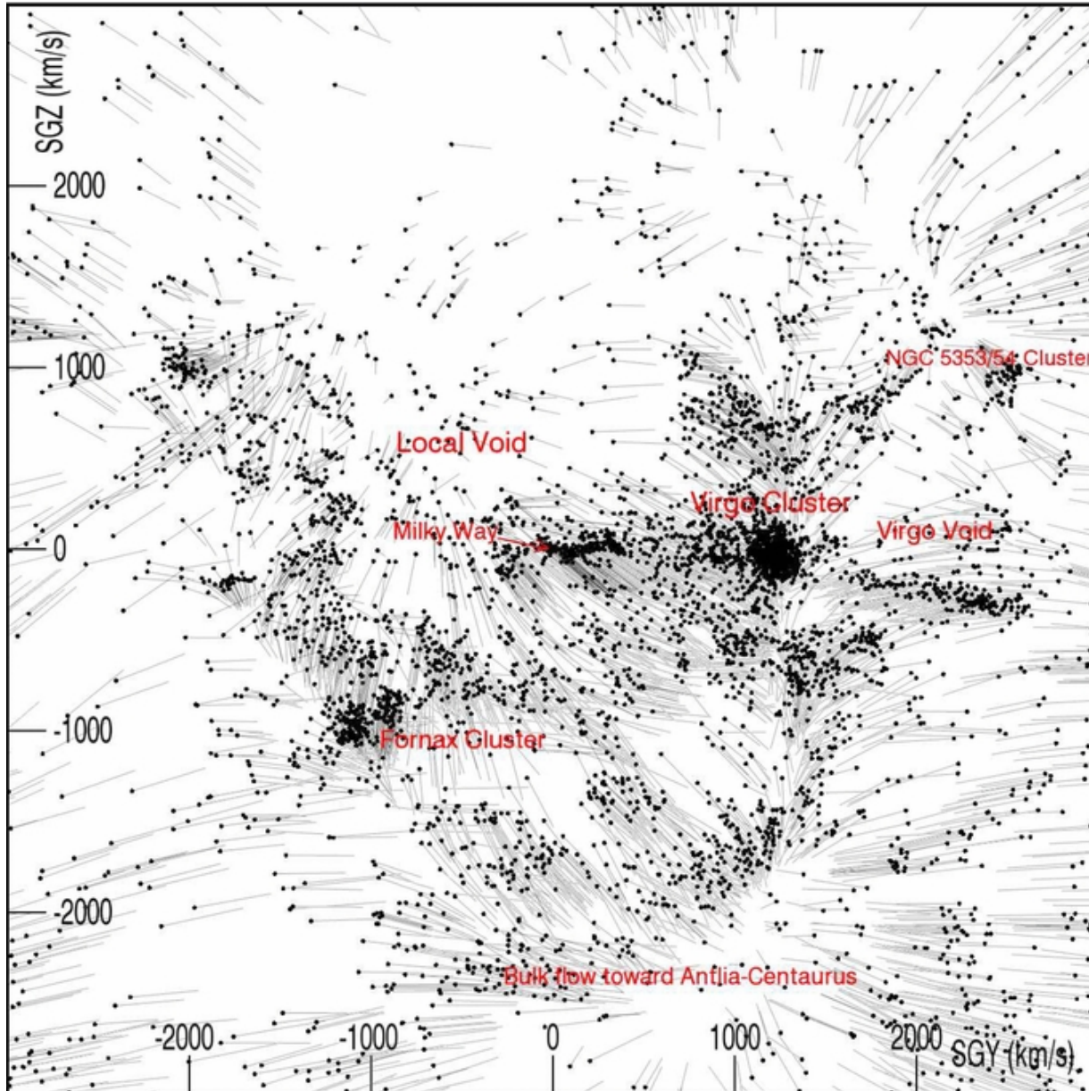
Figure 20. from Cosmography of the Local Universe Courtois et al. 2013 AJ 146 69 doi:10.1088/0004-6256/146/3/69 https://dx.doi.org/10.1088/0004-6256/146/3/69 © 2013. The American Astronomical Society. All rights reserved.
