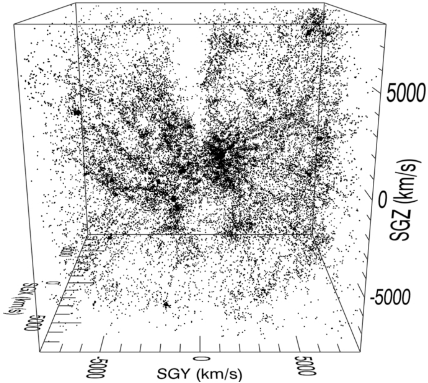
Figure 2. from Cosmography of the Local Universe Courtois et al. 2013 AJ 146 69 doi:10.1088/0004-6256/146/3/69 https://dx.doi.org/10.1088/0004-6256/146/3/69 © 2013. The American Astronomical Society. All rights reserved.
