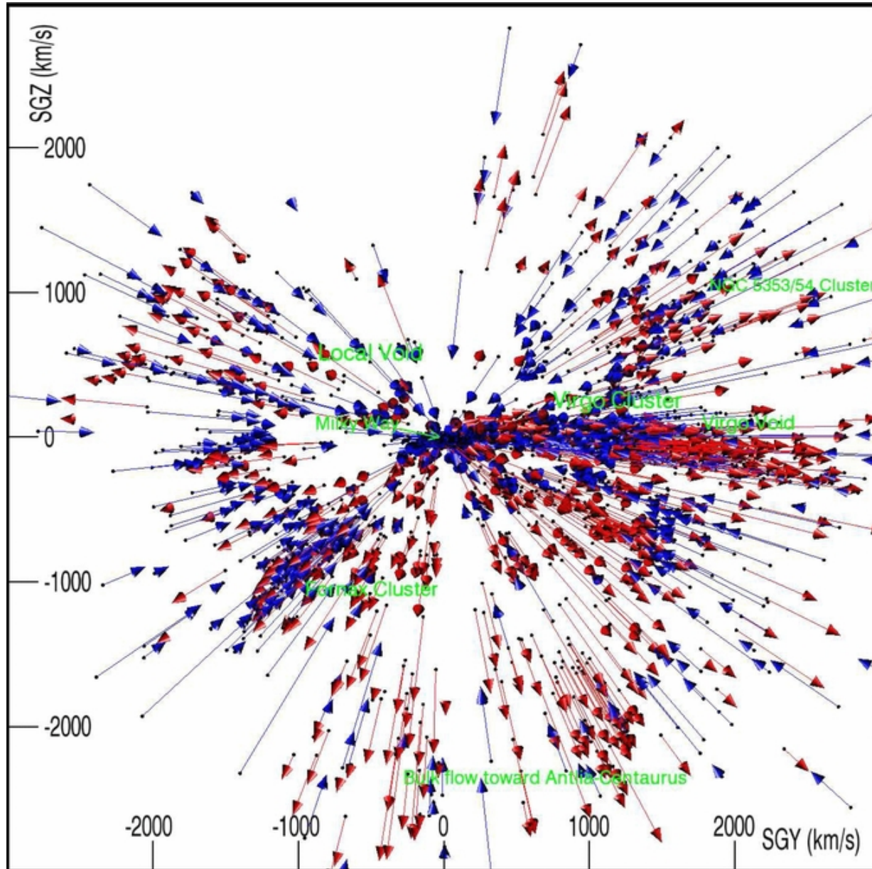
Figure 19. from Cosmography of the Local Universe Courtois et al. 2013 AJ 146 69 doi:10.1088/0004-6256/146/3/69 https://dx.doi.org/10.1088/0004-6256/146/3/69 © 2013. The American Astronomical Society. All rights reserved.
