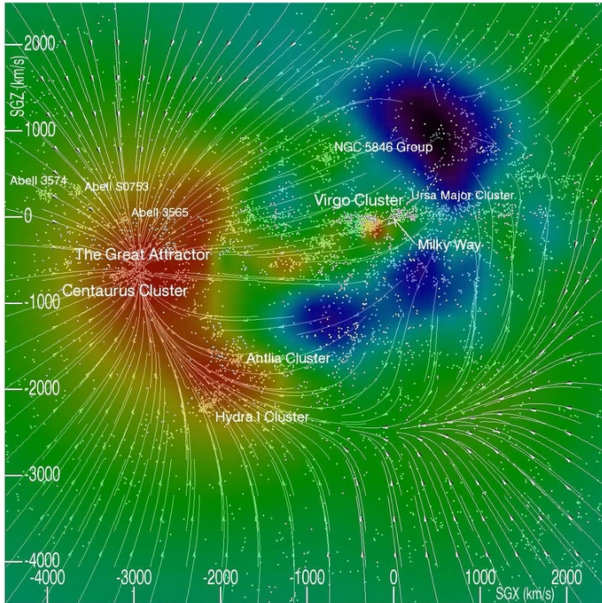
Figure 18. from Cosmography of the Local Universe Courtois et al. 2013 AJ 146 69 doi:10.1088/0004-6256/146/3/69 https://dx.doi.org/10.1088/0004-6256/146/3/69 © 2013. The American Astronomical Society. All rights reserved.
