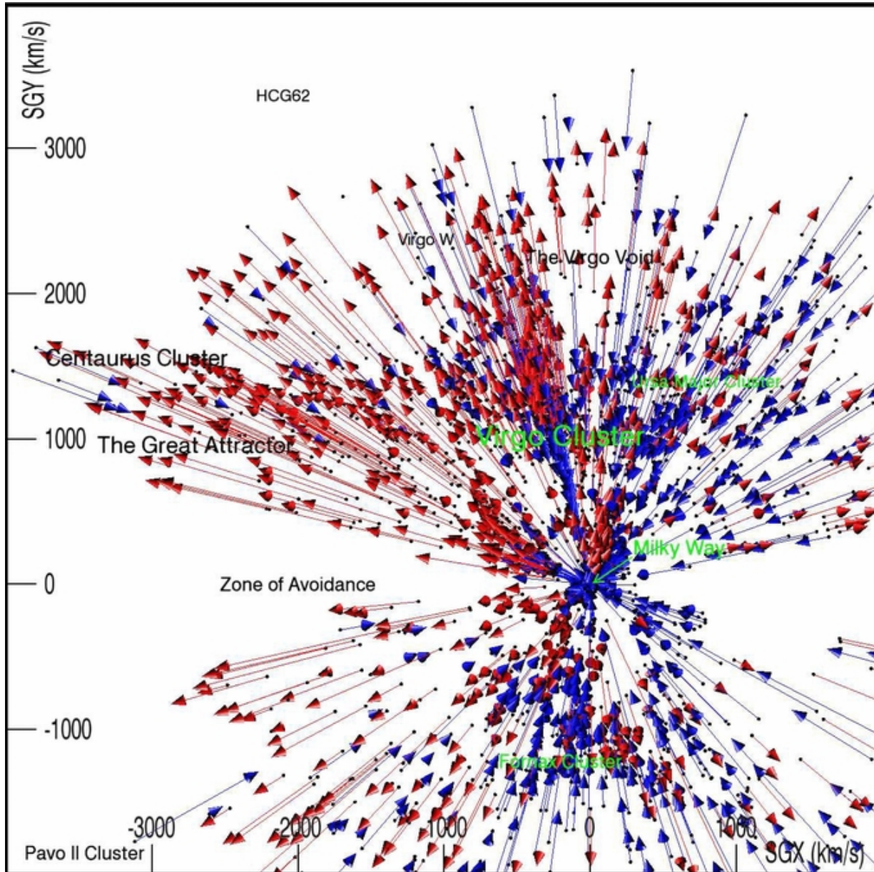
Figure 13. from Cosmography of the Local Universe Courtois et al. 2013 AJ 146 69 doi:10.1088/0004-6256/146/3/69 https://dx.doi.org/10.1088/0004-6256/146/3/69 © 2013. The American Astronomical Society. All rights reserved.
