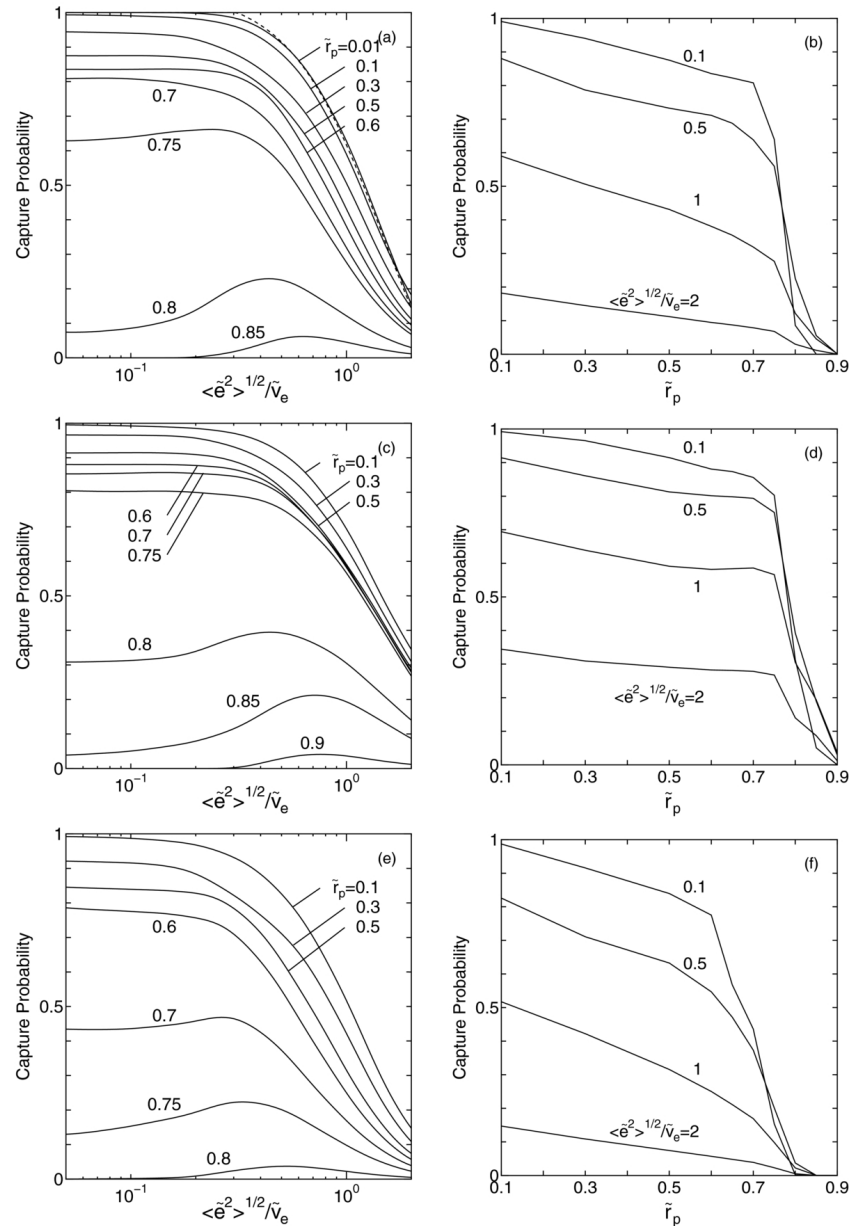
Figure 8. from Accretion Rates of Moonlets Embedded in Circumplanetary Particle Disks Ohtsuki, Yasui, & Daisaka 2013 AJ 146 25 doi:10.1088/0004-6256/146/2/25 https://dx.doi.org/10.1088/0004-6256/146/2/25 © 2013. The American Astronomical Society. All rights reserved.
