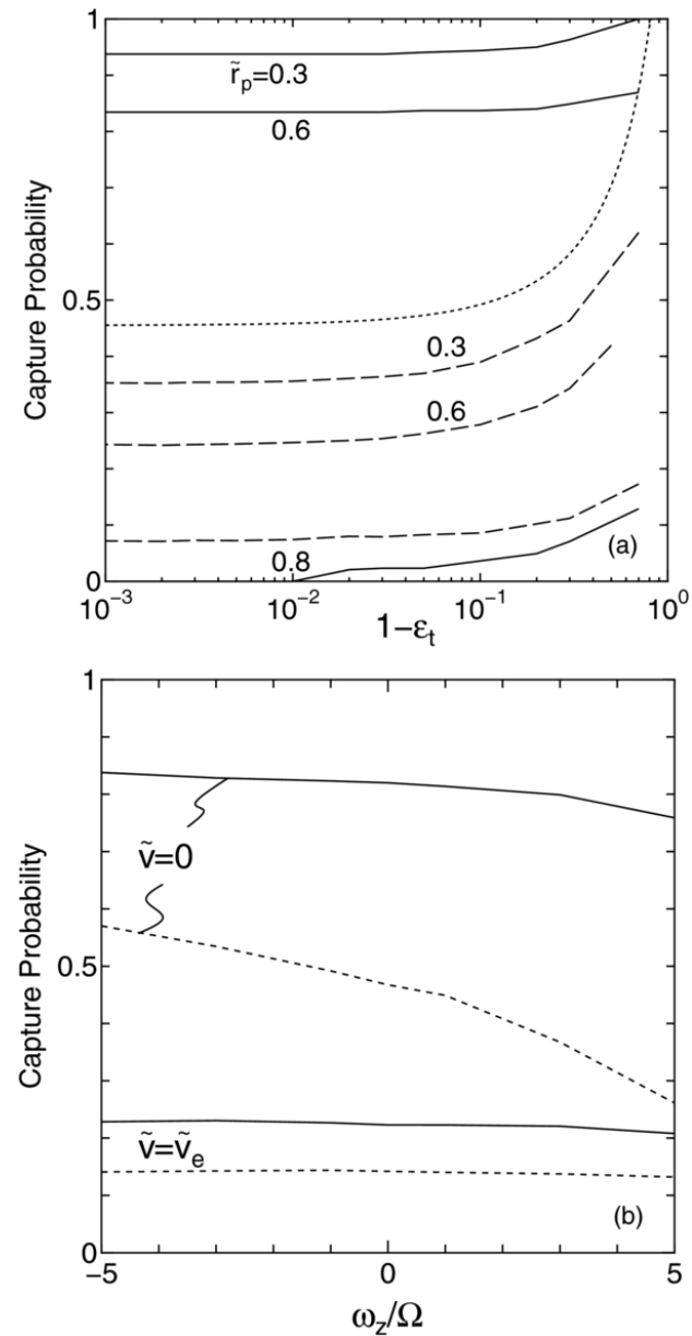
Figure 7. from Accretion Rates of Moonlets Embedded in Circumplanetary Particle Disks Ohtsuki, Yasui, & Daisaka 2013 AJ 146 25 doi:10.1088/0004-6256/146/2/25 https://dx.doi.org/10.1088/0004-6256/146/2/25 © 2013. The American Astronomical Society. All rights reserved.
