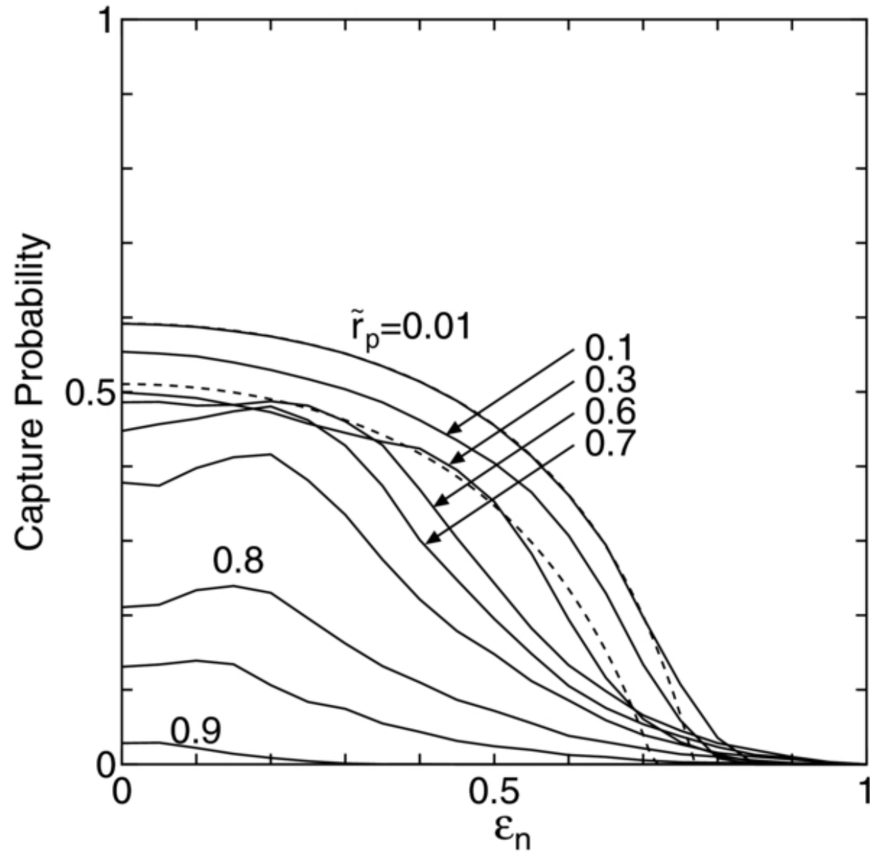
Figure 6. from Accretion Rates of Moonlets Embedded in Circumplanetary Particle Disks Ohtsuki, Yasui, & Daisaka 2013 AJ 146 25 doi:10.1088/0004-6256/146/2/25 https://dx.doi.org/10.1088/0004-6256/146/2/25 © 2013. The American Astronomical Society. All rights reserved.
