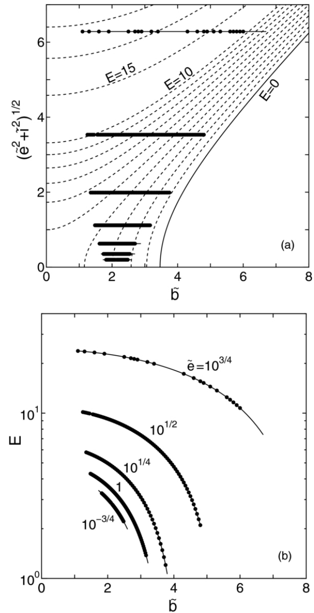
Figure 5. from Accretion Rates of Moonlets Embedded in Circumplanetary Particle Disks Ohtsuki, Yasui, & Daisaka 2013 AJ 146 25 doi:10.1088/0004-6256/146/2/25 https://dx.doi.org/10.1088/0004-6256/146/2/25 © 2013. The American Astronomical Society. All rights reserved.
