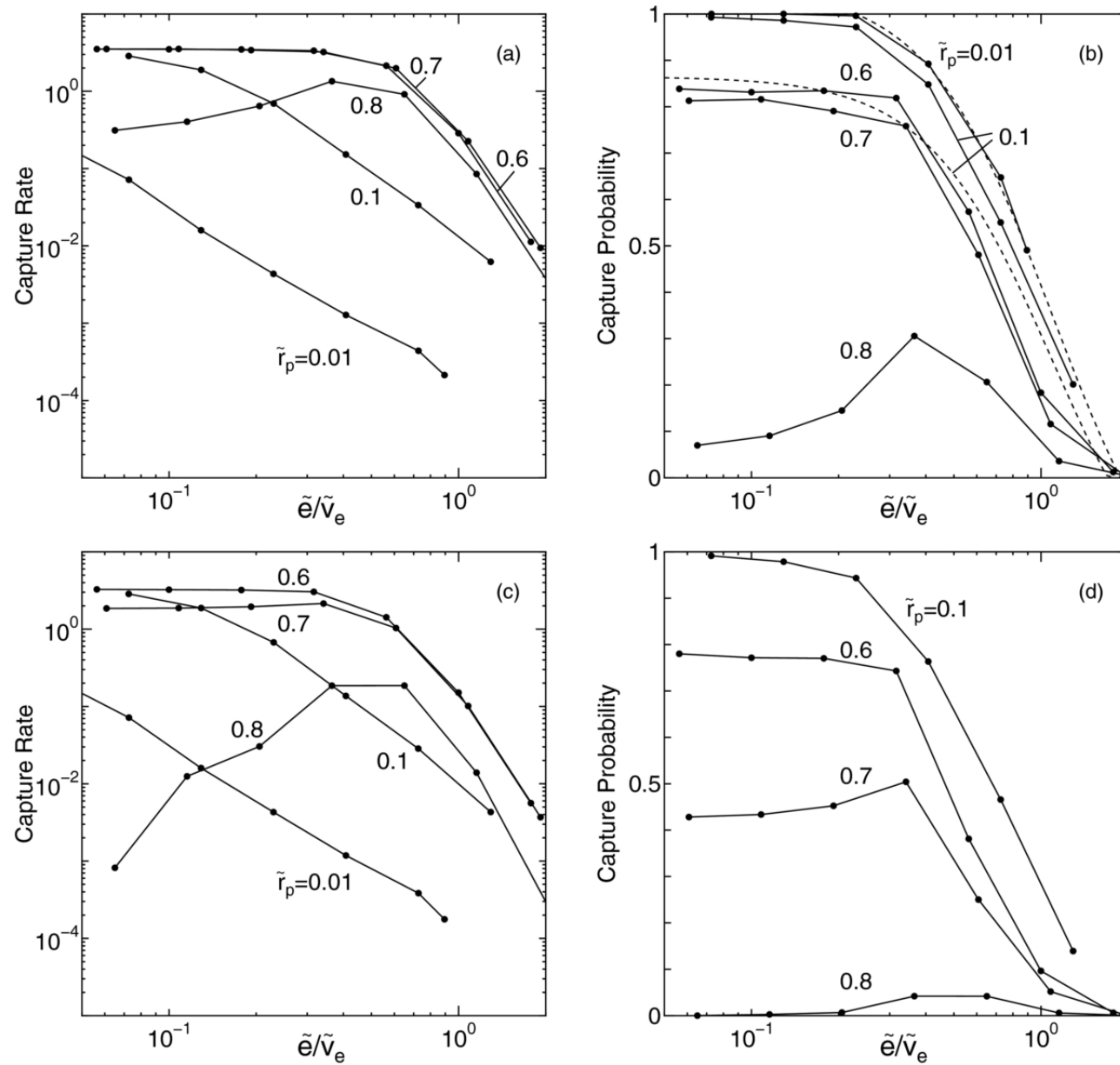
Figure 4. from Accretion Rates of Moonlets Embedded in Circumplanetary Particle Disks Ohtsuki, Yasui, & Daisaka 2013 AJ 146 25 doi:10.1088/0004-6256/146/2/25 https://dx.doi.org/10.1088/0004-6256/146/2/25 © 2013. The American Astronomical Society. All rights reserved.
