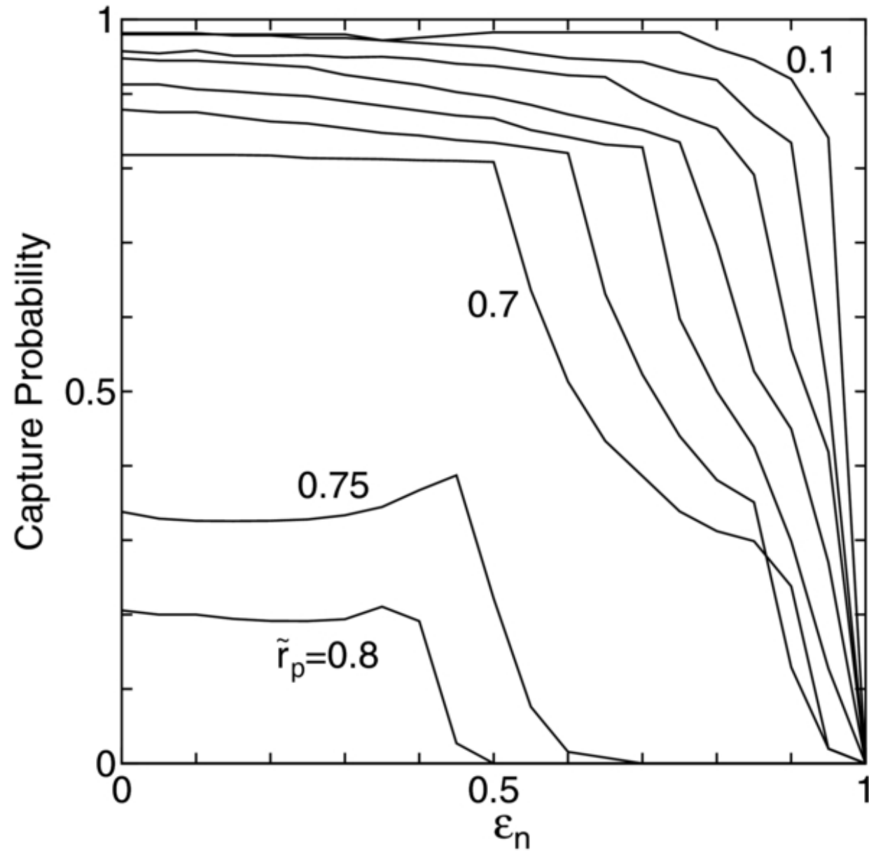
Figure 3. from Accretion Rates of Moonlets Embedded in Circumplanetary Particle Disks Ohtsuki, Yasui, & Daisaka 2013 AJ 146 25 doi:10.1088/0004-6256/146/2/25 https://dx.doi.org/10.1088/0004-6256/146/2/25 © 2013. The American Astronomical Society. All rights reserved.
