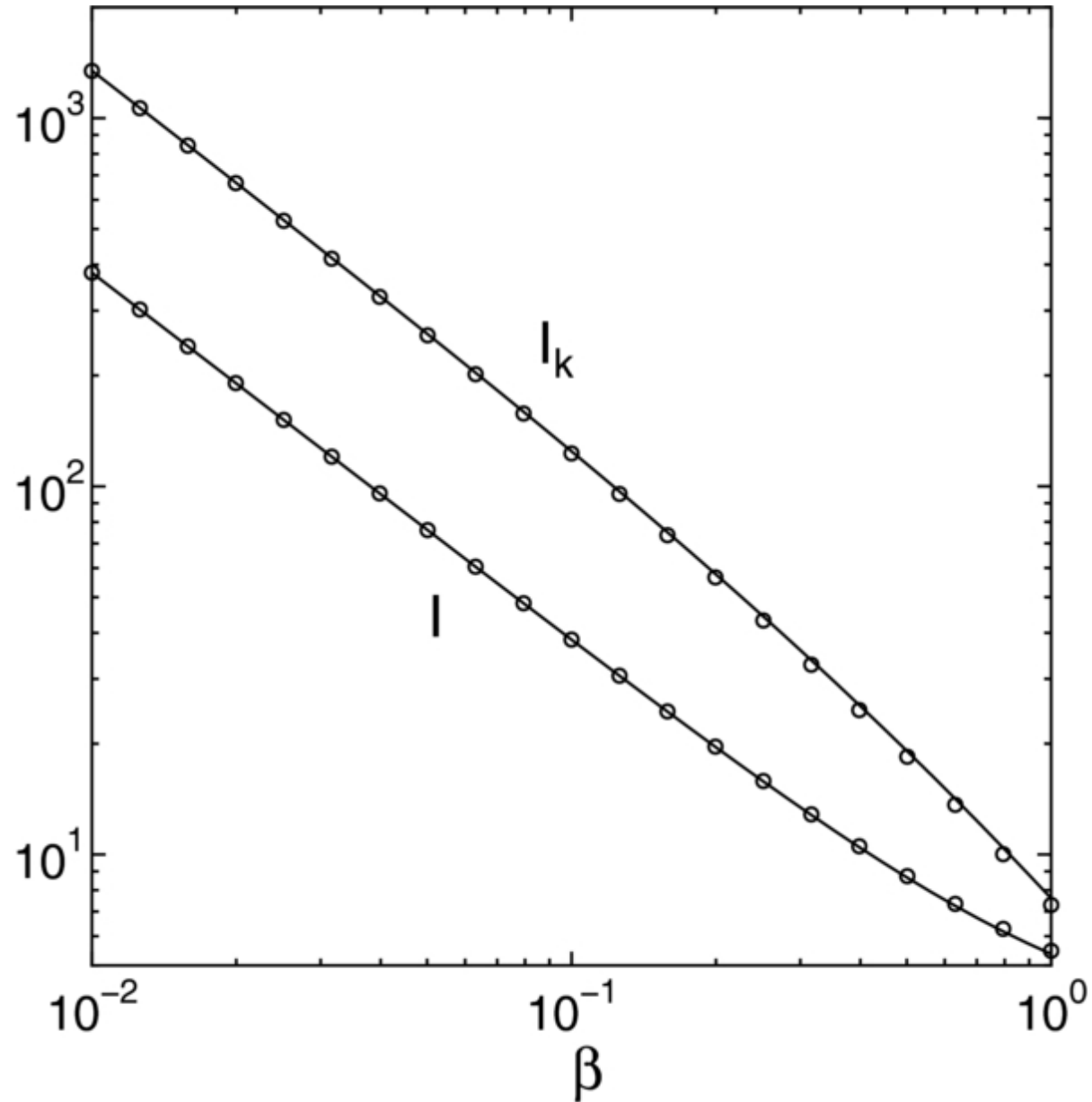
Figure 12. from Accretion Rates of Moonlets Embedded in Circumplanetary Particle Disks Ohtsuki, Yasui, & Daisaka 2013 AJ 146 25 doi:10.1088/0004-6256/146/2/25 https://dx.doi.org/10.1088/0004-6256/146/2/25 © 2013. The American Astronomical Society. All rights reserved.
