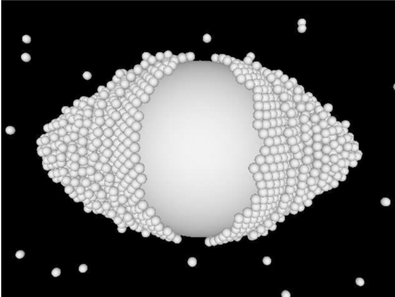
Figure 11. from Accretion Rates of Moonlets Embedded in Circumplanetary Particle Disks Ohtsuki, Yasui, & Daisaka 2013 AJ 146 25 doi:10.1088/0004-6256/146/2/25 https://dx.doi.org/10.1088/0004-6256/146/2/25 © 2013. The American Astronomical Society. All rights reserved.
