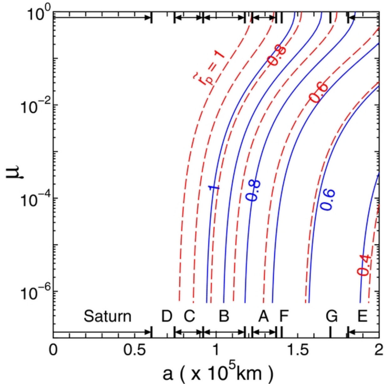
Figure 1. from Accretion Rates of Moonlets Embedded in Circumplanetary Particle Disks Ohtsuki, Yasui, & Daisaka 2013 AJ 146 25 doi:10.1088/0004-6256/146/2/25 https://dx.doi.org/10.1088/0004-6256/146/2/25 © 2013. The American Astronomical Society. All rights reserved.
