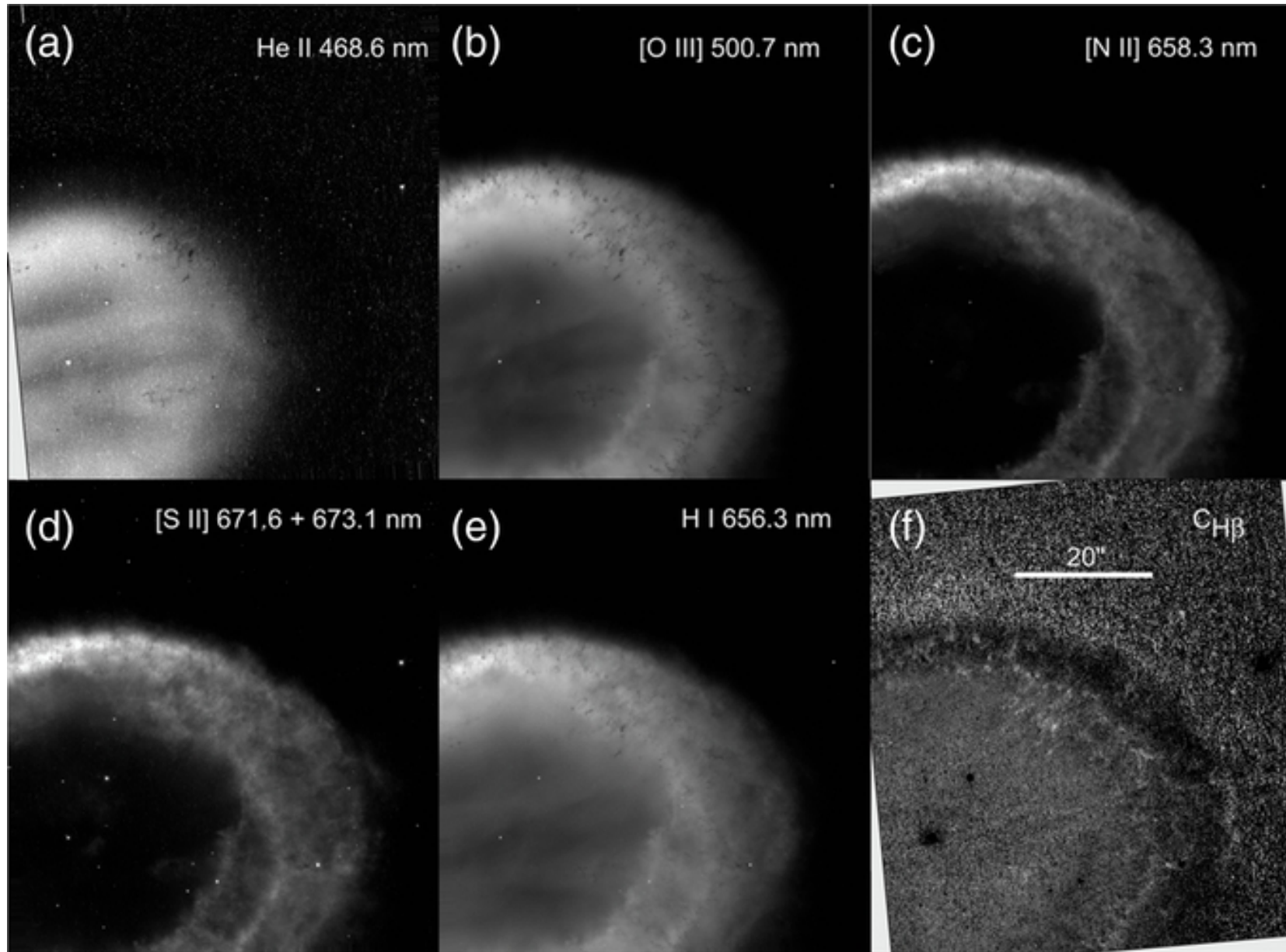
Figure 1. from Studies of NGC 6720 with Calibrated HST/WFC3 Emission-line Filter Images. II. Physical Conditions O'Dell et al. 2013 AJ 145 93 doi:10.1088/0004-6256/145/4/93 https://dx.doi.org/10.1088/0004-6256/145/4/93 © 2013. The American Astronomical Society. All rights reserved.
