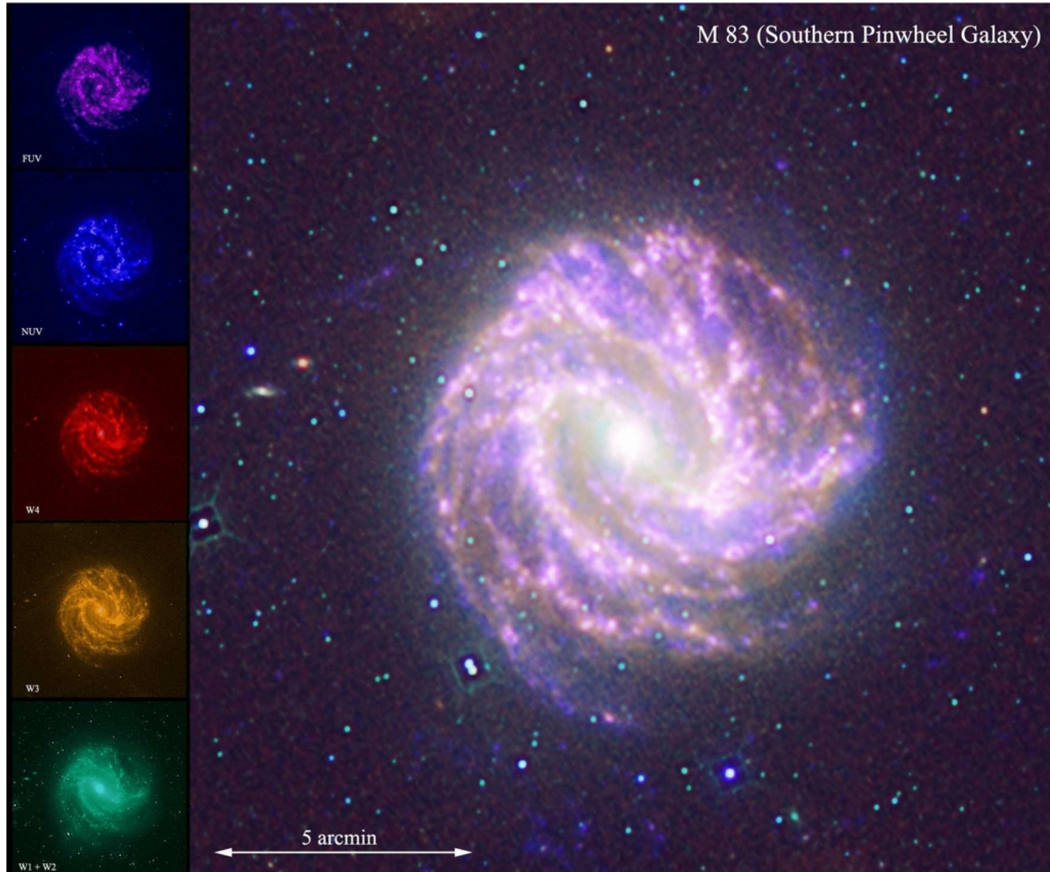
Figure 9. from Extending the Nearby Galaxy Heritage with WISE: First Results from the WISE Enhanced Resolution Galaxy Atlas Jarrett et al. 2013 AJ 145 6 doi:10.1088/0004-6256/145/1/6 https://dx.doi.org/10.1088/0004-6256/145/1/6 © 2013. The American Astronomical Society. All rights reserved.
